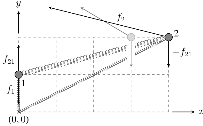
Figure 3: Illustration of the example in Remark 5.16 in the Oxy -plane (in which the motion takes place).
