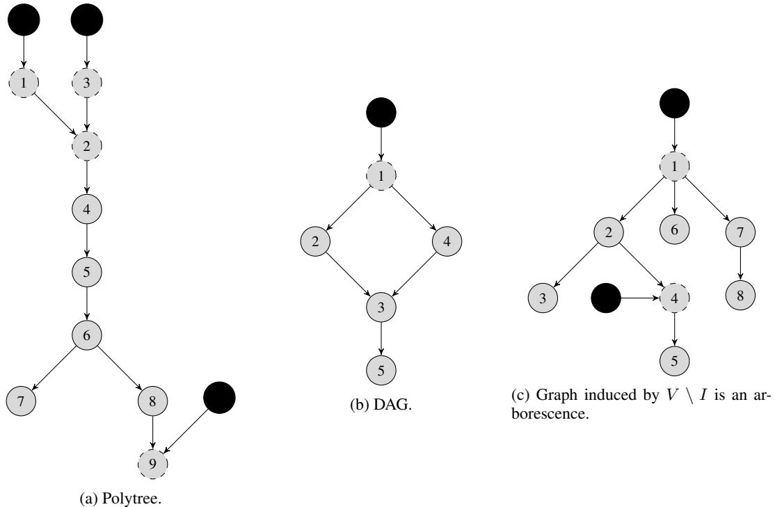
Figure 10: The set I is represented by black vertices and candidate vertices are dashed.
