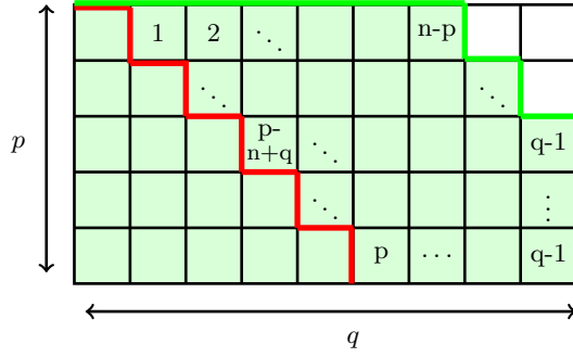
FIGURE 2. The labels in \Lambda(p, q)/\rho , \Lambda(p, q) = (q^{n-q+1}, q-1, \dots, n-p+1) , \rho = (p, \dots, 1) the maximal staircase contained in \Lambda , indicate the column index of \Lambda minus one. The reading word, from right to left and from the top to bottom, defines the reduced word \sigma(\Lambda(p, q), SE) .
