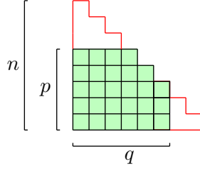
FIGURE 1. The truncated Ferrers shape \Lambda(p, q) , in green, fitting the p by q rectangle so that the staircase D_q of size n is the smallest one containing \Lambda(p, q) . If p \leq q , (p, p-1, \dots, 1) is the biggest staircase inside \Lambda(p, q) .
