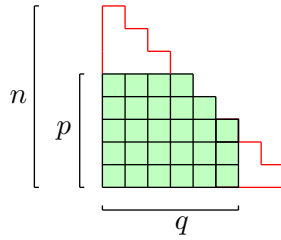
FIGURE 1. The truncated Ferrers shape \Lambda(p, q) , in green, fitting the p by q rectangle so that the staircase D_\varrho of size n is the smallest one containing \Lambda(p, q) . If p \leq q , (p, p-1, \dots, 1) is the biggest staircase inside \Lambda(p, q) .
