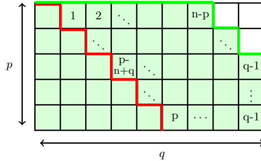
FIGURE 2. The labels in \Lambda(p, q)/\rho , \Lambda(p, q) = (q^{n-q+1}, q-1, \dots, n-p+1) , \rho = (p, \dots, 1) the maximal staircase contained in \Lambda , indicate the column index of \Lambda minus one. The reading word, from right to left and from the top to bottom, defines the reduced word \sigma(\Lambda(p, q), SE) .
