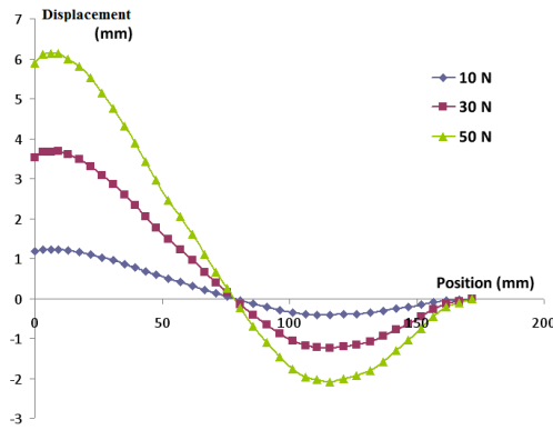
Figure 5. Effect of the boundary condition (from 10 N to 50 N) on the shear wave displacement within the vastus medialis muscle. The profiles are obtained with a fixed frequency (90 Hz) and the muscle properties set to 16 kPa ( C_{10} ).
