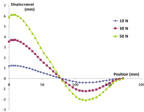
Figure 5. Eft of the boundary condition (from 10 N to 50 N) on the shear wave displacement within the vastus medialis muscle. The profiles are obtained with a fixed frequency (90 Hz) and the muscle properties set to 16 kPa ( C_{10} ).
