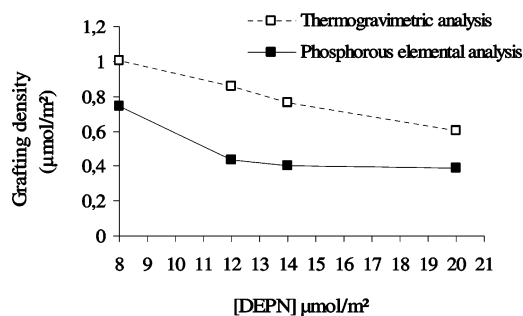
Figure 5. Alkoxyamine grafting densities as a function of DEPN concentration (route II). Silica concentration 2 wt % in toluene. (Acryloxypropyl)trimethoxysilane concentration 12 \mu\text{mol}/\text{m}^2 . Azobisisobutyronitrile concentration 6 \mu\text{mol}/\text{m}^2 . Temperature 70 °C. Reaction time 26 h.
