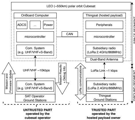
Fig. 2. ThingSat hosted payload: deployed components and architecture.
