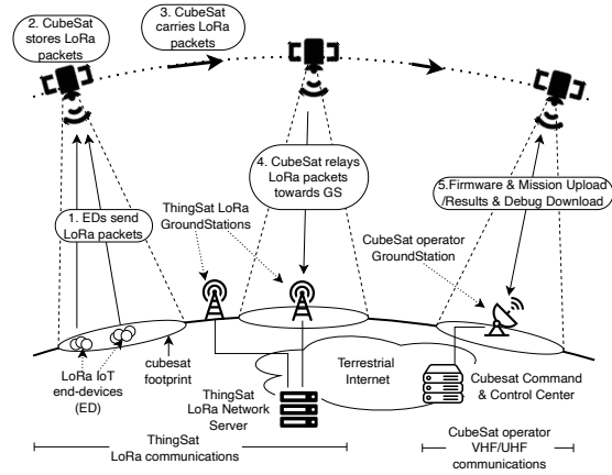
Fig. 3. ThingSat in-orbit communication patterns.
