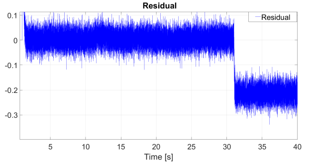
Fig. 4. Residual fault indicator
