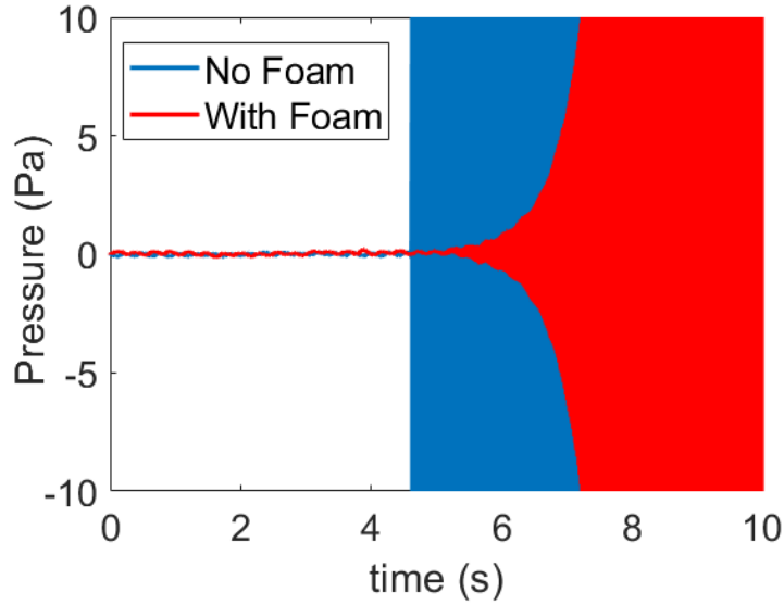
Figure 25: Time history of the pressure signal recorded at the upsurge of instability, in case of absence (blue curve) and presence (red curve) of the 12 mm foam layer.
