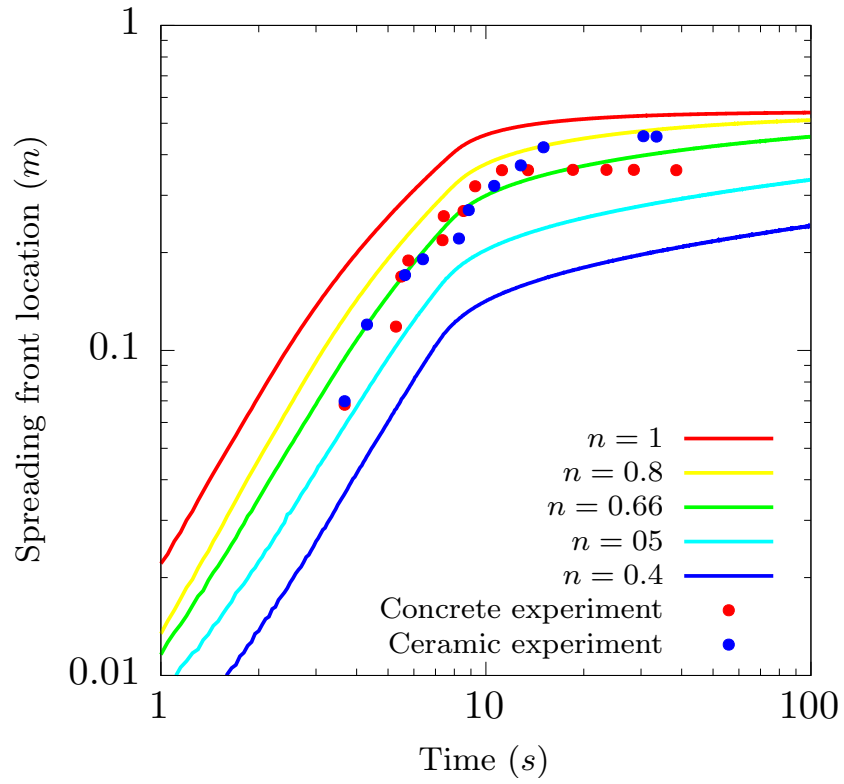
Figure 9: Simulated front progress for Arr = 7.10^{-3} , \tau_y = 100 Pa and different values of the fluid index n , and experimental results for the VEU7 test, for both concrete and ceramic substrate channels. log-log representation of fig. 8
