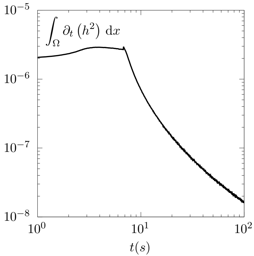
Figure 11: Evolution of \int_{\Omega} (h^2) dx , for the simulation with n = 0.66 and \tau_y = 200 Pa . It shows that the movement of the melt slows down quickly once corium source stops at t = 7.7s .
