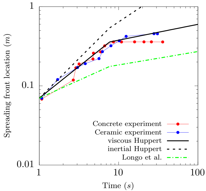
Figure 6: Experimental front position evolution and its comparison to self-similar solutions from [32, 33] for various geometries. We assume from this comparison that the process of corium spreading is mainly viscous during corium inlet feeding.
