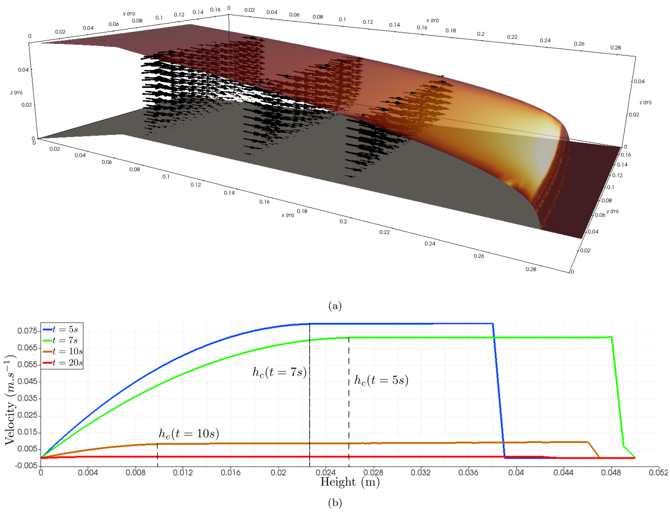
Figure 12: (a) Tridimensional reconstruction of the velocity. The top surface color represents height-averaged temperature. (b) Velocity profiles along the z -axis at t = 5\text{ s} (during melt supplying), t = 7\text{ s} (close to the end of melt supplying), t = 10\text{ s} (after the end of melt supply, toward melt front stop) and t = 20\text{ s} at x = 12\text{ cm} and y = 10\text{ cm}
