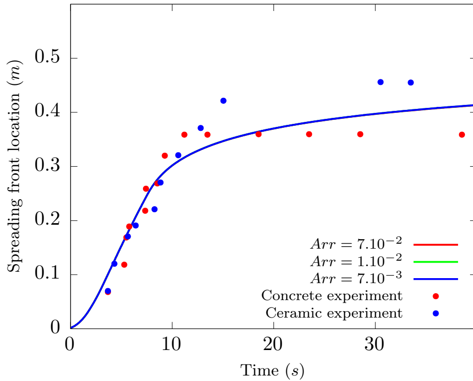
Figure 7: Simulated front progress for n = 1 , \tau_y = 100 Pa and different values of the Shaw model coefficient Arr , and experimental results for the VEU7 test, for both concrete and ceramic substrate channels.
