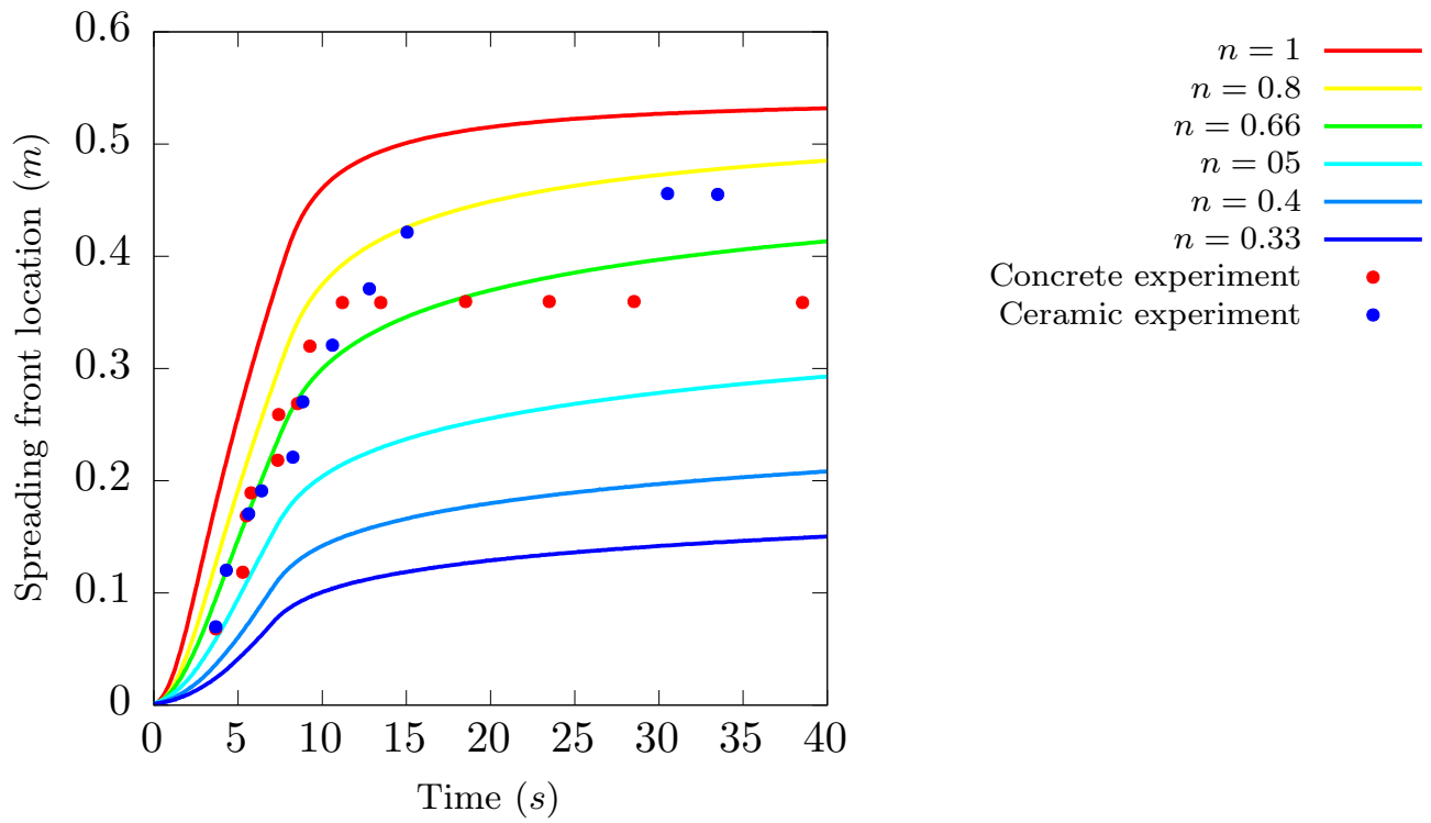
Figure 8: Simulated front progress for Arr = 7.10^{-3} , \tau_y = 100 Pa and different values of the fluid index n , and experimental results for the VEU7 test, for both concrete and ceramic substrate channels.
