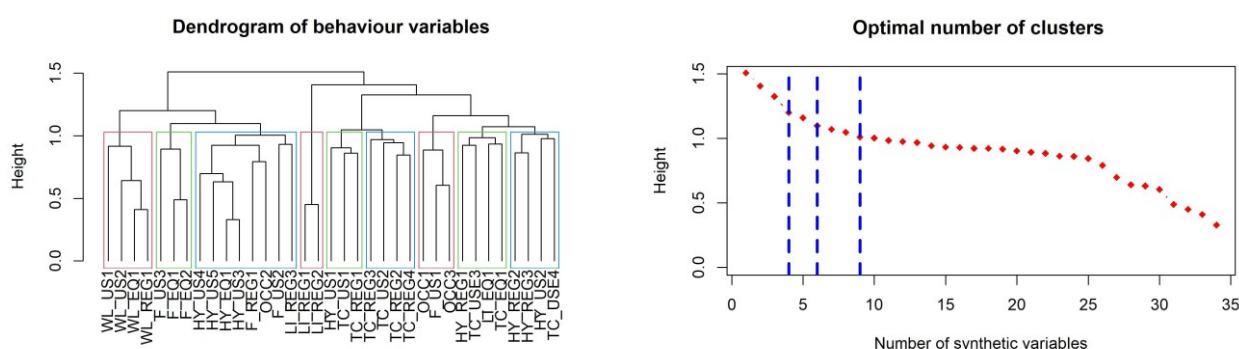
(A) Dendrogram of behaviour variables. The height of a cluster C = A \cup B is defined as h(C) = d(A, B)
