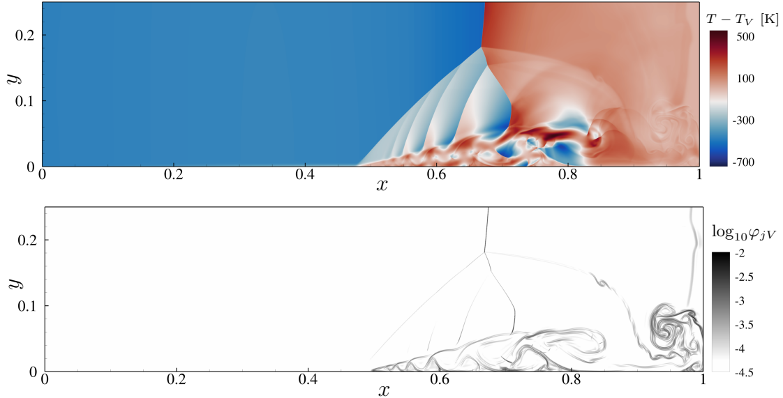
Figure 5: Instantaneous visualization of temperatures difference (top) and logarithm of \varphi_{jV} (bottom), at t = 1 ms, for the viscous shock tube in thermochemical non-equilibrium.
