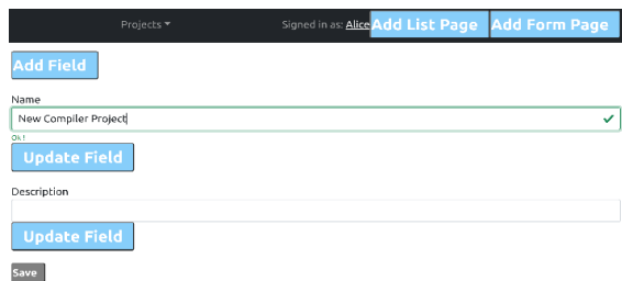
Figure 4: A form page with some modification actions (blue buttons)
