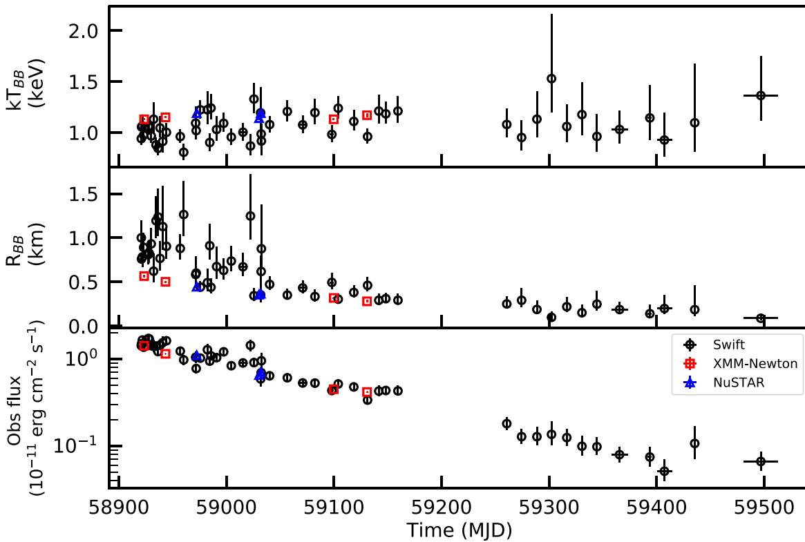
Figure 4. Temporal evolution of the blackbody temperature (top panel) and radius (middle panel). The latter is evaluated for a distance of 4.8 kpc (see Section 3.2 for more details). The bottom panel shows the temporal evolution of the observed flux in the 0.3–10 keV energy range.
