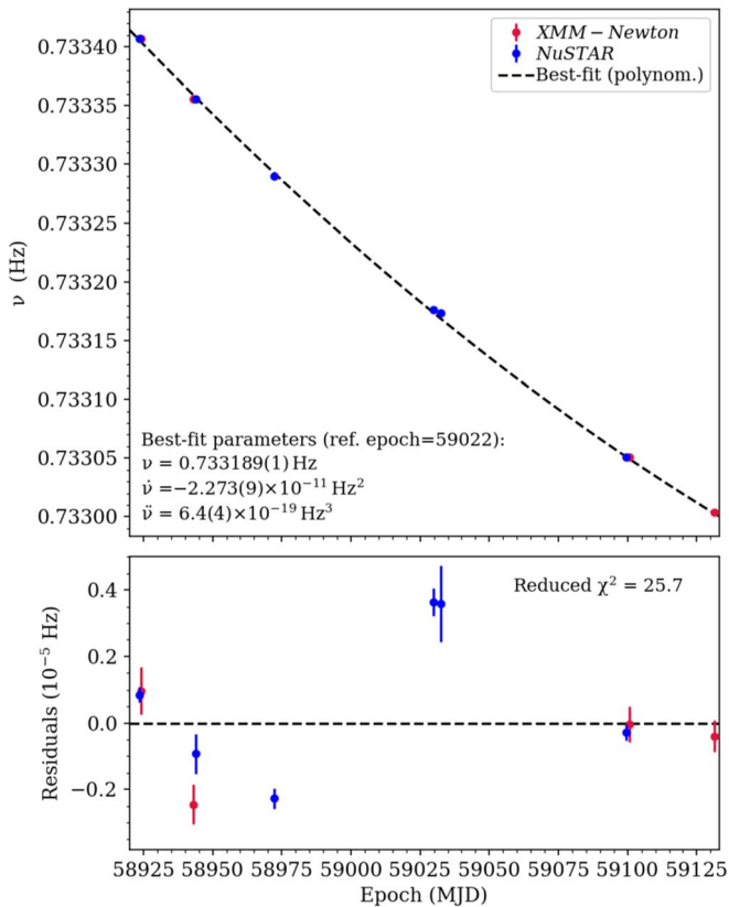
Figure 5. TEMPO-derived values of the spin frequency \nu in each observation. The epochs of the XMM-Newton and NuSTAR observations are shown as red and blue filled circles. Error bars correspond to the 1\sigma uncertainties reported by TEMPO. Black dashed-dotted lines are the best-fit models for \nu(t) (see text in Section 3.4). As evidenced by the large reduced \chi^2 values we measured (provided in the top right corner of the bottom panel), the \nu(t) solutions poorly fit the data. This is explained by the large timing noise present in Swift J1818 and the simplicity of our models.
