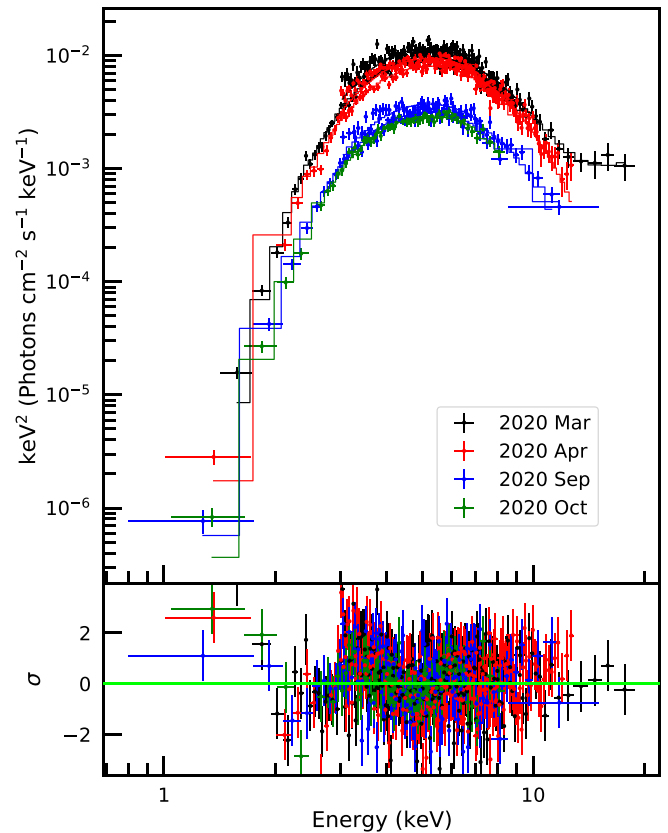
Figure 3. E^2 f(E) unfolded spectra of Swift J1818 from XMM-Newton and NuSTAR observations. In the fit, we adopted a model consisting of two blackbodies, except for the 2020 March spectra where we included a power law ( \chi^2_\nu = 1.41 for 607 dof). Post-fit residuals in units of standard deviations are shown in the bottom panel.
