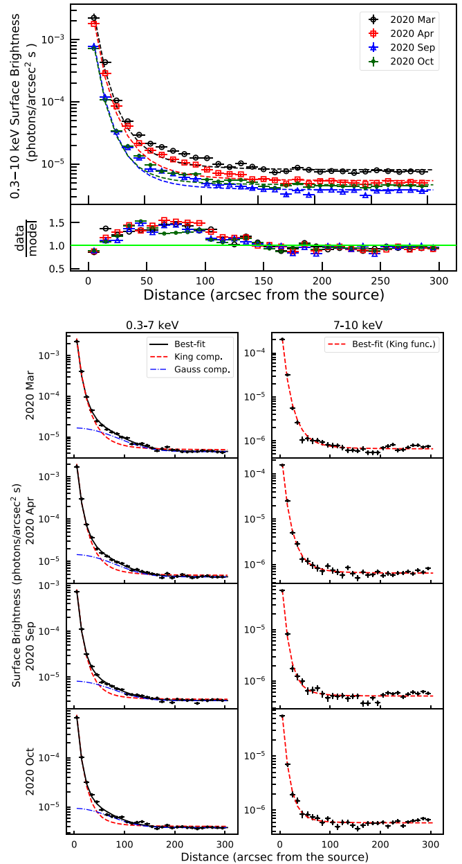
Figure 1. Top panel: Observed X-ray surface brightness up to a radial distance of 300'' in the 0.3–10 keV energy range extracted from the four XMM-Newton observations (the error bars are smaller than the size of the markers). The dashed lines represent the best-fit PSF model. The ratio between the data and the best-fit model is plotted in the lower subpanel. Bottom panels: Observed X-ray surface brightness up to a radial distance of 300'' in two different energy bands, 0.3–7 keV (left) and 7–10 keV (right). The best-fitting models are superimposed.
