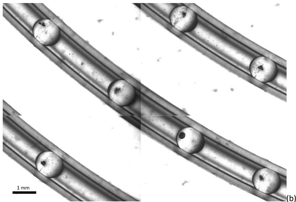
Figure 3: Sulfathiazole in water droplets generated at 70°C in GPL107 oil and cooled to 10°C, tubing of 1mm inner diameter: (a): full spiral reconstruction from 180 pictures; (b) zoom on (a) at the junction of four pictures, zone indicated by the square in (a).
