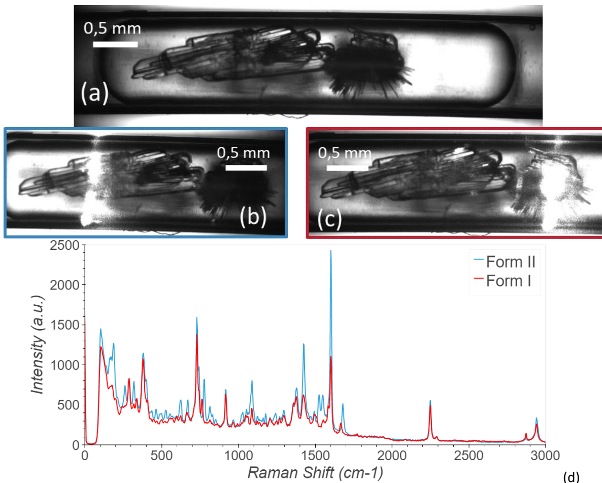
Figure 5: (a) Plug of acetonitrile containing Rimonabant crystals, generated from saturated solution at 70°C and cooled to 30°C; (b) Laser focused on the left crystal; (c) Laser focused on the right crystal; (d) Raman spectra corresponding to the left crystal (Form II) and the right crystal (Form I).
