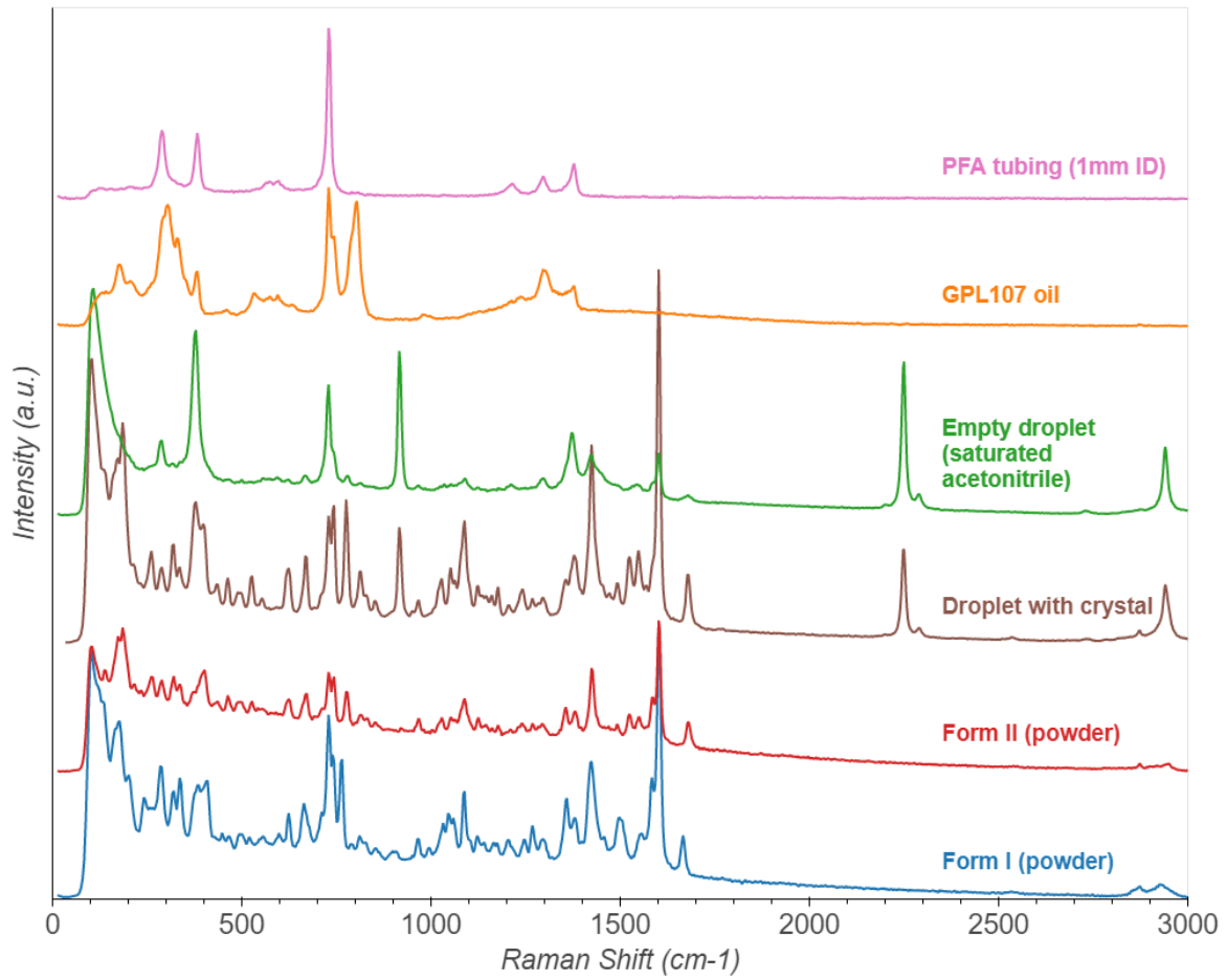
SIF Figure 4 : Raman spectra of GPL 107 oil, an empty droplet of Rimonabant in acetonitrile, a droplet of acetonitrile containing a Rimonabant crystal (form II) and references of Rimonabant form I and II from powder
