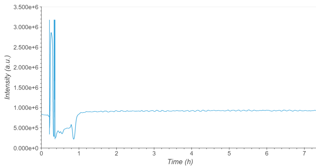
SIF Figure 6 : UV signal as a function of time of the diluted solution of Aripiprazole in acetonitrile
