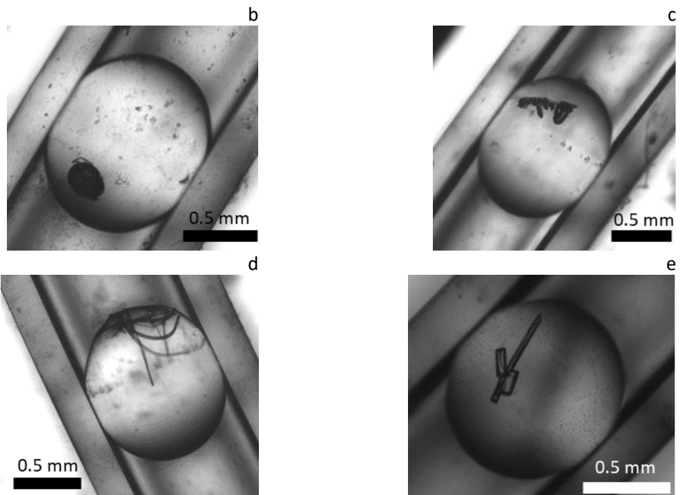
Figure 8: (a) Percentage (and number of crystals) of Sulfathiazole forms II, III, IV, mixture II+IV and unknown U1, U2 and U3 among the droplets containing crystals with -0.5^{\circ}\text{C/h} and -5^{\circ}\text{C/h} ramps in water from 70^{\circ}\text{C} to 10^{\circ}\text{C} . ( b, c, d and e) Crystals habits of Sulfathiazole obtained in water, mainly for (b) forms II and IV; (c) unknown U1; (d) unknown U2; (e) unknown U3.
