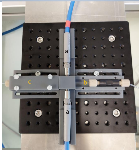
SIF Figure 1 : UV holder: The central part serves to hold UV-solarised optical fiber (a) aligned on both sizes of the quartz capillary (b). A printed cover (c) is added on both sides to prevent the capillary moving and breaking.
