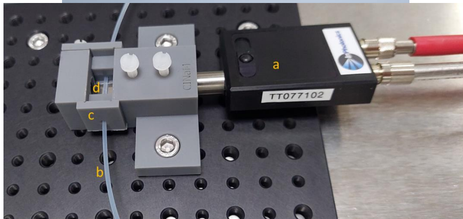
SIF Figure 2: Raman probe holder: the Raman probe (a) position can be adjusted in y, to focus the beam on the middle of the capillary (b). The capillary is hold by a mobile piece (c) to adjust its position in z. It can also manually be moved in x. A mirror is fixed in the bottom of the observation zone (d).
