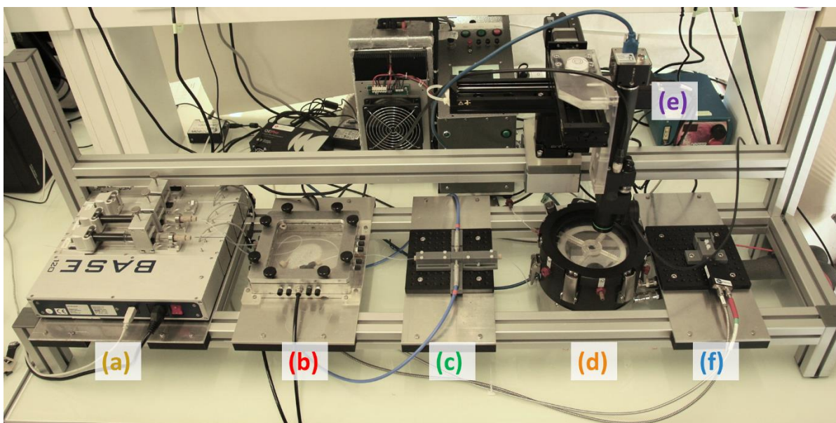
Figure 1 : Microfluidic platform: (a) Syringes and pumps; (b) Solutions and droplet generation with temperature control; (c) UV characterisation; (d) Droplet storage and cooling; (e) Optical characterisation; (f) Raman characterisation
