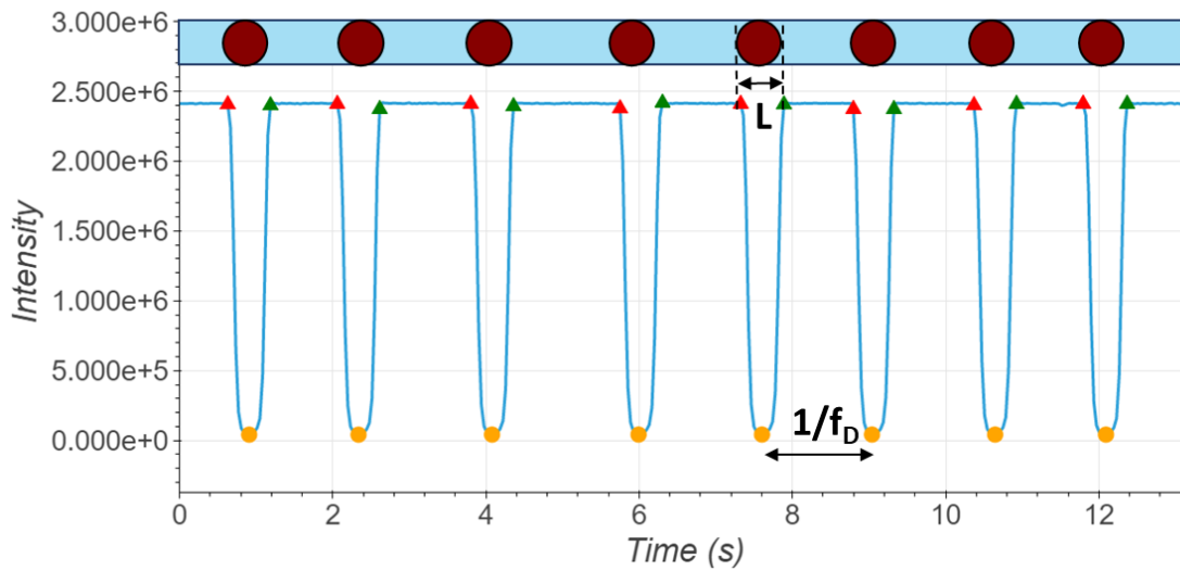
SIF Figure 3 : Real-time recording of light intensity at 280 nm of circulating droplets. L and f_D are respectively the length of the droplets and their frequency.
