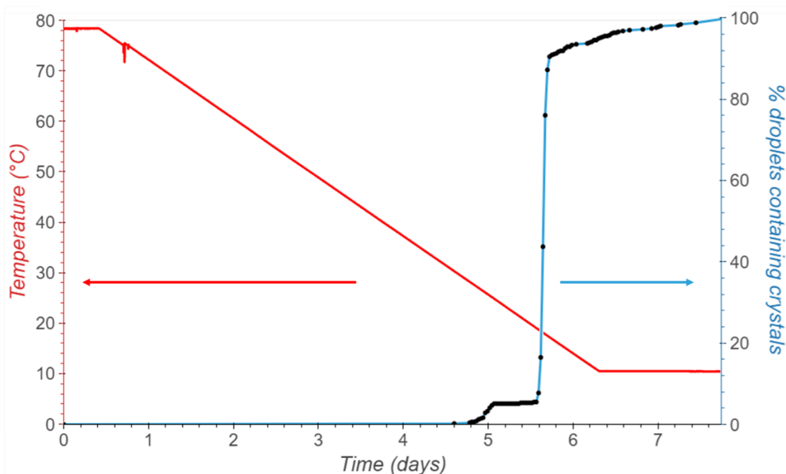
Figure 7: Percentage of droplets of water containing crystals of Sulfathiazole as a function of time (blue) and temperature profile as a function of time (red). (a) for a fast-cooling ramp ( -5^{\circ}\text{C}/\text{h} ); (b) for a slow cooling ramp ( -0.5^{\circ}\text{C}/\text{h} )
