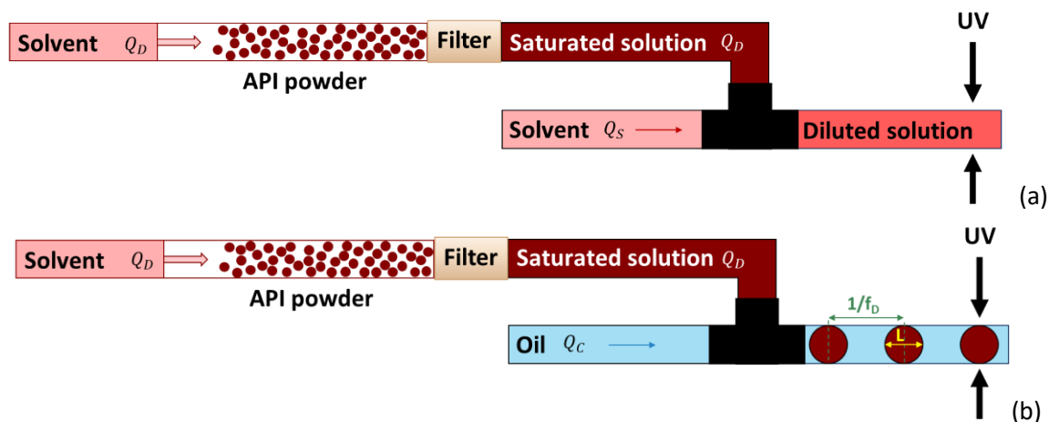
Figure 2: Saturated solution generation followed by (a) dilution for solubility measurements; (b) droplet generation in oil, Q_D , Q_S and Q_C are respectively the discontinuous form flow (saturated solution), the dilution solvent flow and the continuous form flow (oil). L and f_D are respectively the length of the droplets and their frequency.
