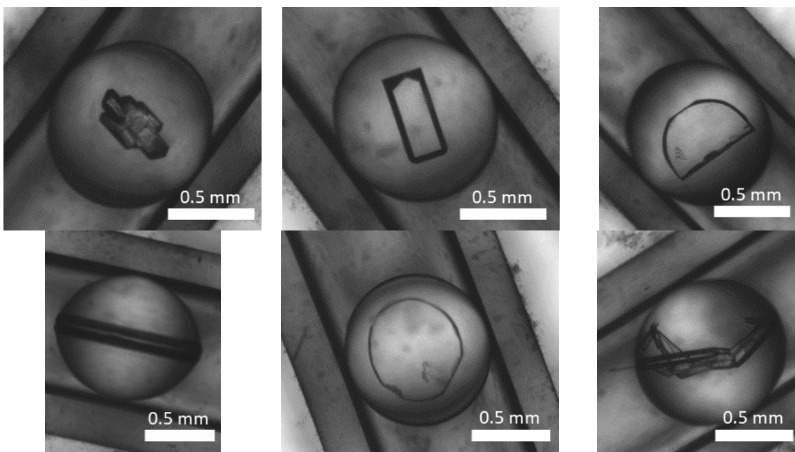
SIF Figure 11: Crystals habits of Sulfathiazole obtained in acetonitrile with a -5^{\circ}\text{C} ramp from 70^{\circ}\text{C} to 10^{\circ}\text{C}
