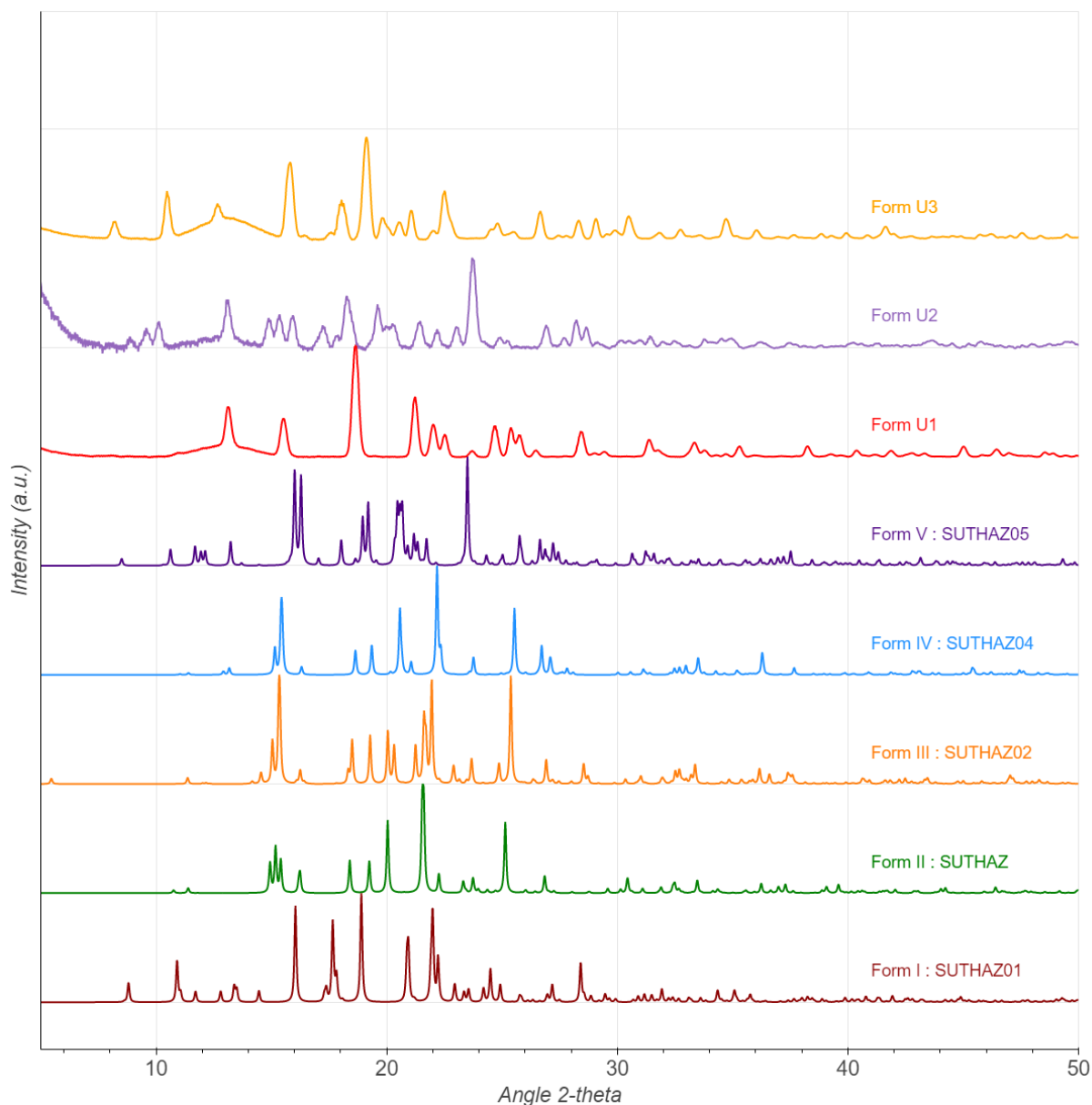
SIF Figure 8 : XRD patterns of different crystalline forms of Sulfathiazole. SUTHAZ, SUTHAZ01, SUTHAZ02, SUTHAZ04 and SUTHAZ05 are references from the Cambridge Structural Database. U1, U2 and U3 were measured on crystals obtained in water droplets.
