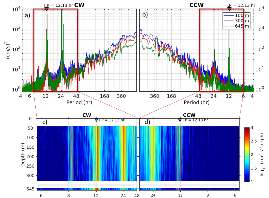
Figure 3. (a, b) Rotary spectra of velocity time series at 100, 300, and 645 m averaging over groups of four adjacent frequencies (2 hr resolution velocities). x-axis is period in hour (4–720 hr), y-axis is energy (in \text{cm}^2/\text{s}^2 ). CW, clockwise; CCW, counterclockwise. (c, d) Vertically coordinated frequency spectrum for the complex horizontal current: left (CW) clockwise rotation and right (CCW) counterclockwise rotation. Periods in hours. Velocities were high-pass filtered with a 50 hr-period cutoff (Section 2.1).
