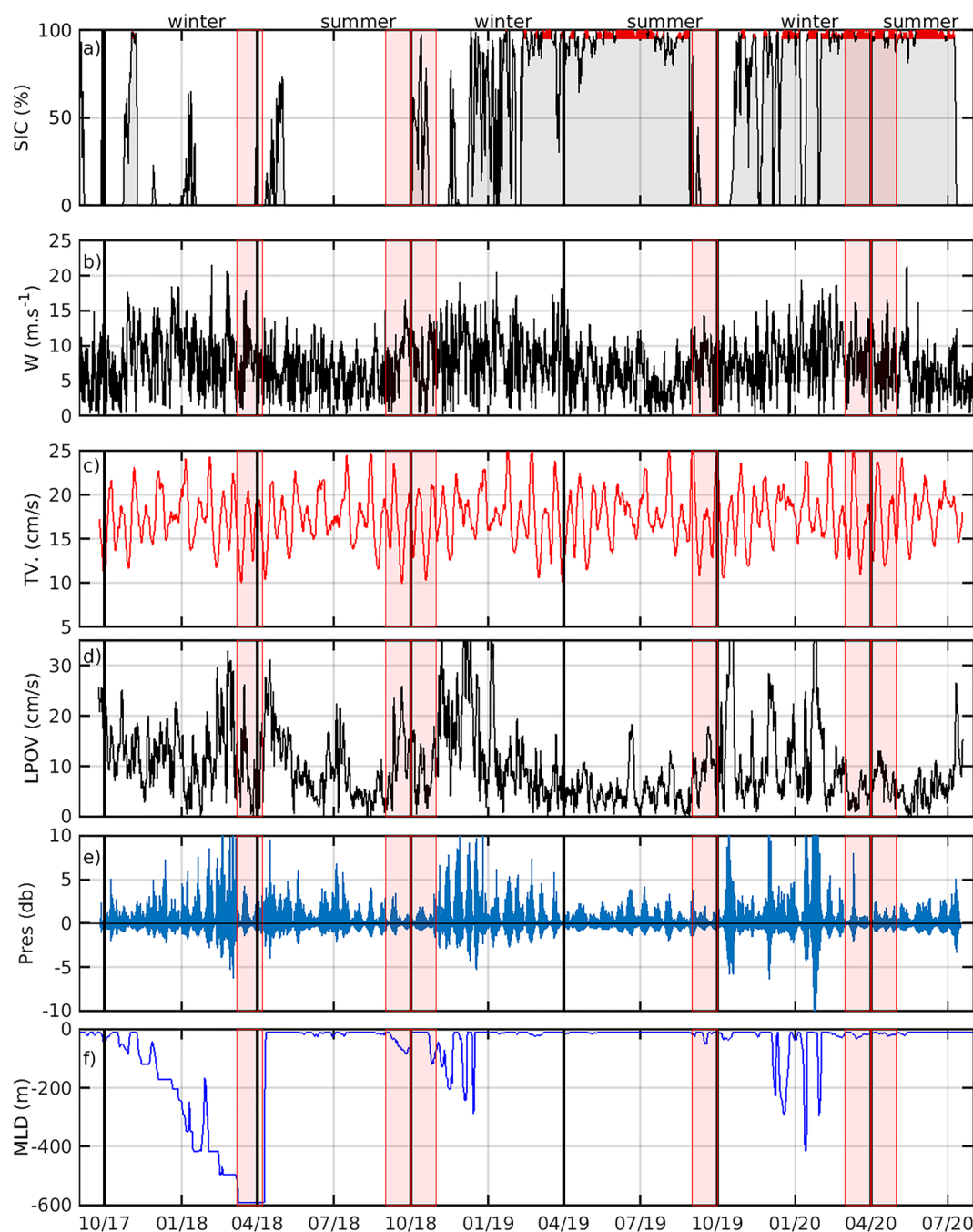
Figure 4. Time series of (a) sea ice concentration (SIC), (b) wind amplitude (W), (c) tidal velocity amplitude (TV), (d) 50-hr low-pass filtered ocean velocity amplitude at 100 m (LPOV), (e) 50-hr high-pass filtered pressure at 345 m and (f) mixed layer depth from PSY4. Selected periods are shaded in red. (Summer: April–September, winter: October–March).
