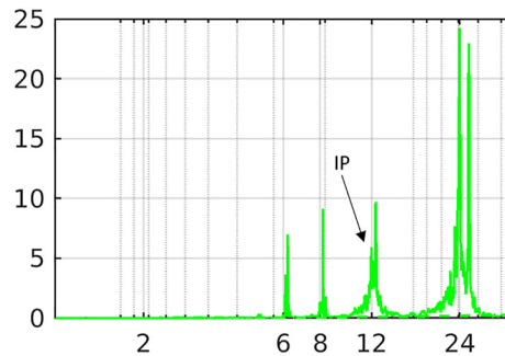
Figure A2. Spectral content averaging over groups of 10 adjacent frequencies (sampling time 10 min) of pressure. x -axis is period in hr and y -axis (db)^2 . The dotted line close to the x -axis shows the 95% confidence interval. IP stands for inertial period: 12.13 hr.
