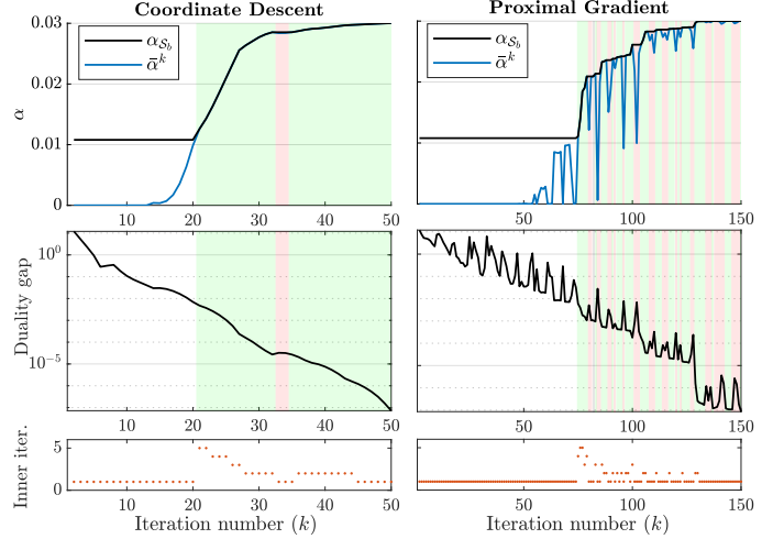
Fig. 3: Evolution of \bar{\alpha}^k and \alpha_{S_b} (top), the duality gap G^k (middle), and the number of inner refinement iterations performed by Alg. 1 (bottom), as a function of the outer iteration number k . Green, grey (very rare) and red backgrounds depict respectively the improvement , indecisive , and no-improvement situations. The initial white region corresponds to a “burn-in” phase where \bar{\alpha}^k < \alpha_{S_b} = \alpha_{\Delta_A} . Indeed, here \alpha_{S_b} has been initialized with \alpha_{\Delta_A} which is known.
