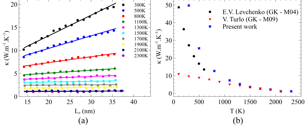
Figure 13: (a) \kappa as a function of the simulation box length for the considered temperatures. Symbols are the numerical results. Lines are the corresponding fits. (b) Bulk thermal conductivity results as a function of temperature compared with the values reported by Levchenko et al. [48] and Turlo et al. [34]. These two authors computed \kappa with the Green-Kubo approach, using Mishin 2004 (M04) [49] and Purja Pun and Mishin 2009 (M09) [31] potentials for Ni.
