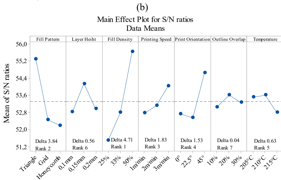
Fig. 5 Main Effects Plot of Young modulus (MPa) obtained from Minitab: (a) for means values, (b) for Signal to Noise ratios (S/N).
