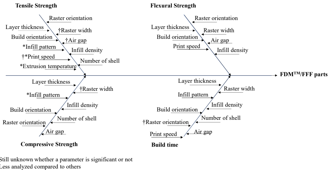
Fig. 1 A fishbone diagram to illustrate the main effect of process parameters on FDM™/FFF part.
