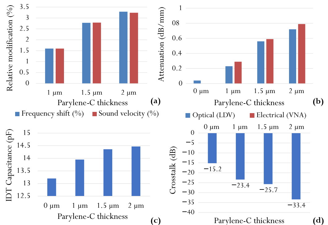
Figure 7. Various sensor characteristics vs. parylene coating thickness: frequency shift and sound velocity variation (a); attenuation (b); IDT capacitance (c); crosstalk (d).
