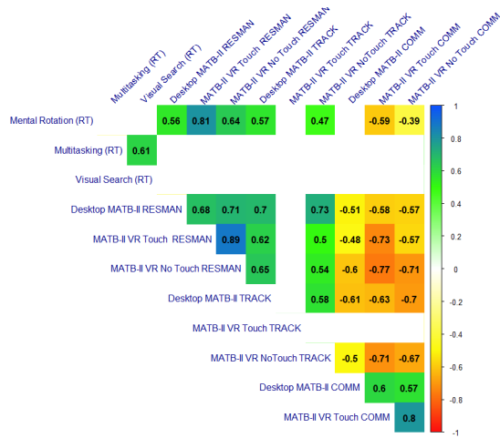
Figure 13: Correlation Matrix of the performances in the three MATB-II variants and during the three neuropsychological tasks. Only significant results are displayed.
