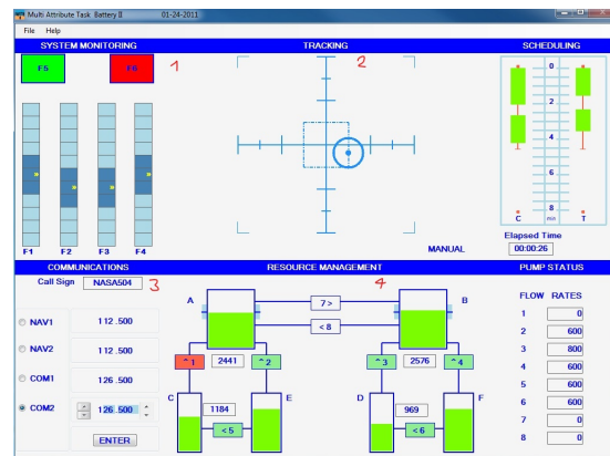
Figure 1: Interface of the original desktop MATB-II.
