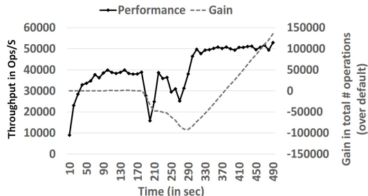
Figure 1: The effect of reconfiguration on the throughput of the system. If the new workload persists for greater than a certain duration (where the gain curve becomes positive), then reconfiguration should be done, else it is better to stay with the earlier configuration.
