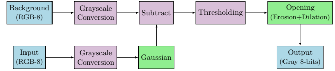
Figure 9. Pipeline for foreground extraction using algorithms and views.
