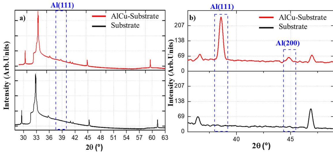
FIG. 1: X-ray diffractograms for an AlCu film (100 nm) deposited on LiNbO 3 (red curve) and for a raw LiNbO 3 substrate (black curve), obtained by grazing mode (GIXRD) left figure (a) and \theta-2\theta mode right figure (b)
