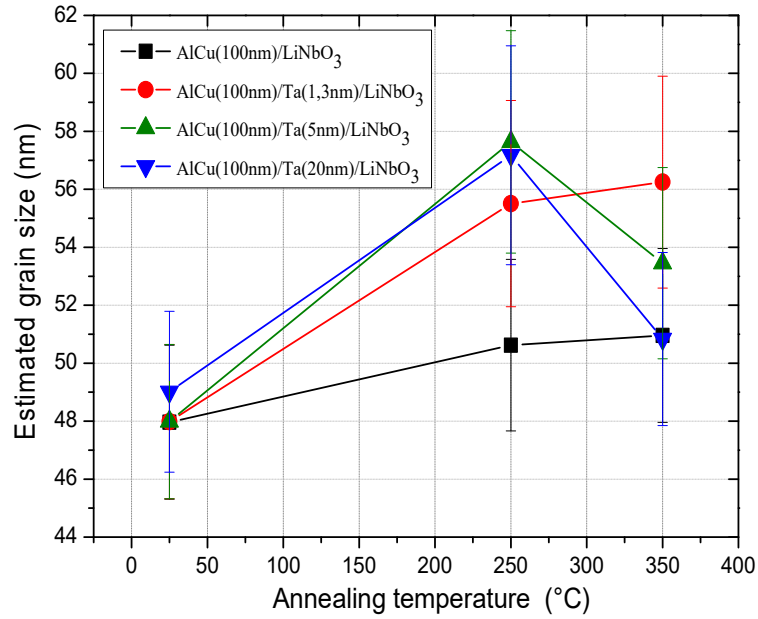
FIG. 2: Evolution of the GS as a function of Ta underlayer thicknesses and temperature of the heat treatment. Thickness of AlCu 2% is 100nm, and Ta underlayer thicknesses are 0, 1.3, 5 and 20nm.
