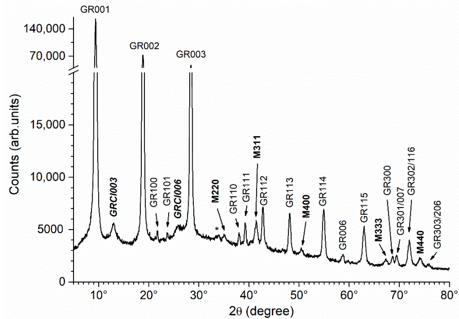
Figure 3. XRD pattern of the precipitate obtained without addition of bacteria or organic compounds, after 1 week of ageing at RT. GR = \text{GR}(\text{SO}_4^{2-}) , GRC1 = \text{GR}(\text{Cl}^-) and M = magnetite, with the corresponding Miller index. * = unidentified peak.
