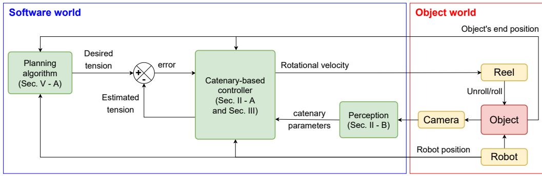
Fig. 1. Control logic block diagram of our proposed method for visual-based tension control scheme.
