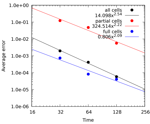
(a) Frank's Spheres convergence results, fixed timestep \Delta t = 10^{-4} . (b) Frank's Spheres convergence results varying timestep and mesh size.
