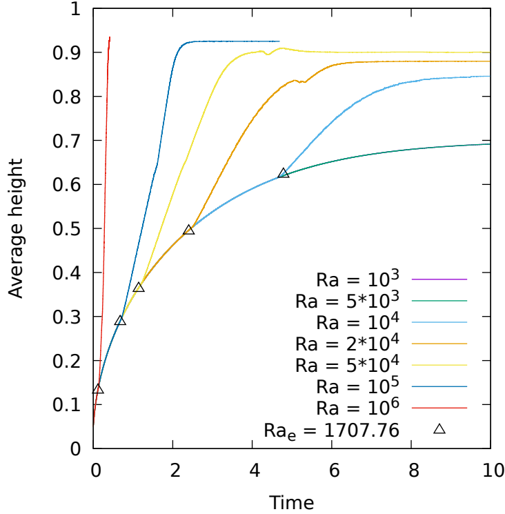
Figure 18: Rayleigh–Bénard instability with a melting boundary. Average height evolution for different Rayleigh numbers
