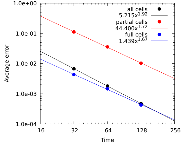
(a) Frank's Spheres convergence results, fixed timestep \Delta t = 10^{-4} . (b) Frank's Spheres convergence results varying timestep and mesh size.
