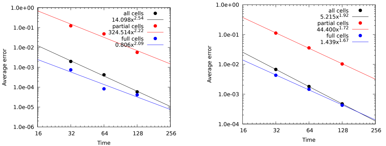
(a) Frank's Spheres convergence results, fixed timestep \Delta t = 10^{-4} . (b) Frank's Spheres convergence results varying timestep and mesh size.
