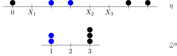
FIGURE 3.1. An example of \eta and its corresponding \hat{\omega}^\eta in an periodic setting.
