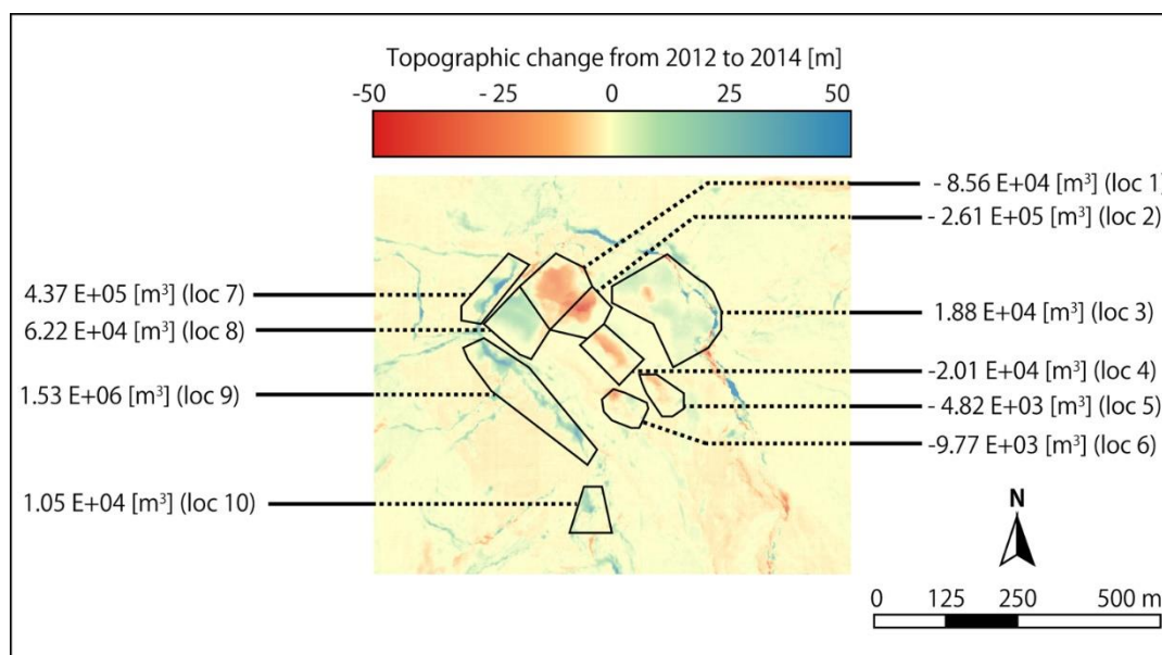
Figure 4. Topographic change from 2012 to 2014. These data show the vents opening and the “split in two” of the dome, as well as the areas between the crater rim and the dome, where the topography increased, arguably due to exploded material deposition. These changes emphasize the changes that are >2.5 \text{ m} (i.e., in blue on the map), valued above the overall RMSE and the RMSE of the outside structure. This procedure may erase some of the minor variations, but it is aimed at eliminating the false positives from the dataset.
