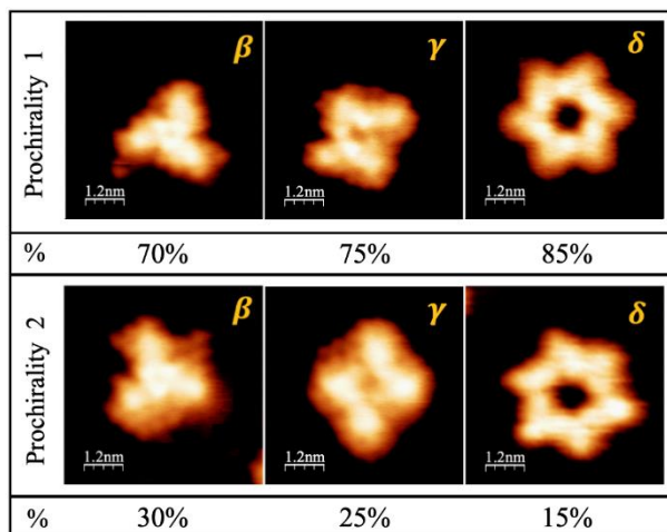
Figure 5: STM images showing the two prochiralities and their relative abundance observed for the \beta , \gamma and \delta -structures obtained after deposition of the molecule R -BrPhINDO on Cu(111).
