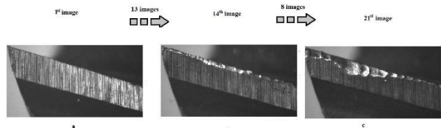
Figure 8. Images taken at successive times during processing showing the stages of tool wear [86].
