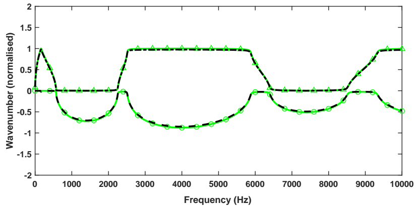
Fig. 15. Comparison of dispersion curves obtained by AWI and WFEM for a bi-material periodic beam under small perturbation condition when the unit-cell length is unknown. ( \Delta —) real part of the wavenumber obtained by AWI, ( \circ —) imaginary part of the wavenumber obtained by AWI, (---) real part of the wavenumber obtained by WFEM, (---) imaginary part of the wavenumber obtained by WFEM.
