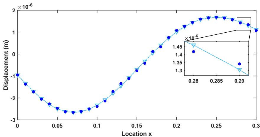
Fig. 8. Operational deflection shape at 400Hz. (▽ ---) uniform perfect samples, (●) uniform small perturbed samples.
