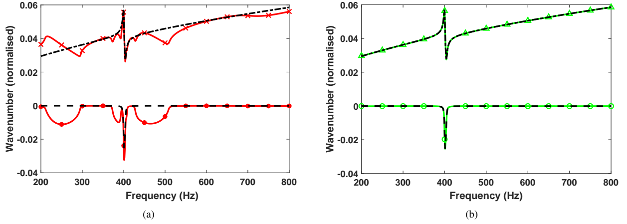
Fig. 9. Dispersion curves comparison for a homogeneous beam with TMDs under uniform sampling and small perturbation condition: (a) INCOME and WFEM; (b) AWI and WFEM. ( \times —) real part of the wavenumber obtained by INCOME, ( \bullet —) imaginary part of the wavenumber obtained by INCOME, ( \Delta —) real part of the wavenumber obtained by AWI, ( \circ —) imaginary part of the wavenumber obtained by AWI, (—) real part of the wavenumber obtained by WFEM, (---) imaginary part of the wavenumber obtained by WFEM.
