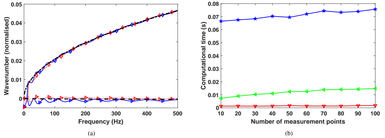
Fig. 5. (a) Comparison of propagative wavenumber obtained by IWC for a homogeneous beam using the complete and incomplete data set in perfect condition, respectively. ( \diamond —) real part of the wavenumber obtained by IWC using the complete data set, ( \triangleright —) imaginary part of the wavenumber obtained by IWC using the complete data set, ( \diamond - - -) real part of the wavenumber obtained by IWC using the incomplete data set, ( \triangleright - - -) imaginary part of the wavenumber obtained by IWC using the incomplete data set, (—) real part of the wavenumber obtained by WFEM, (- -) imaginary part of the wavenumber obtained by WFEM. (b) Computational time comparison between IWC, INCOME, and AWI as a function of the measurement points. ( \star —) computational time of IWC, ( \nabla —) computational time of INCOME, ( \leftarrow —) computational time of AWI.
