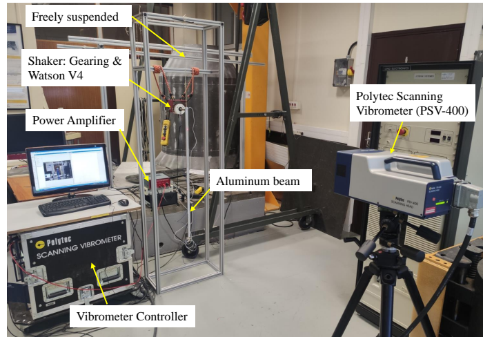
Fig. 16. Experiment set-up for measuring the vibratory field of the aluminum beam
