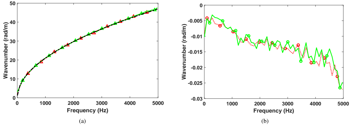
Fig. 19. Comparison of wavenumber obtained by AWI using the complete and incomplete data set: (a) real part of wavenumber; (b) imaginary part of wavenumber. ( \triangle —) real part of the wavenumber obtained by AWI using the complete data set, ( \circ —) imaginary part of the wavenumber obtained by AWI using the complete data set, ( \triangle ---) real part of the wavenumber obtained by AWI using the incomplete data set, ( \circ ---) imaginary part of the wavenumber obtained by AWI using the incomplete data set, (---) real part of the wavenumber obtained by WFEM.
