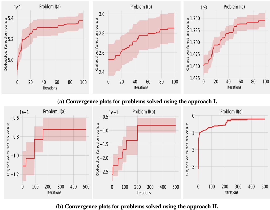
Fig. 5 The obtained optimization convergence plots for problems solved using the approaches I and II. (results of 10 runs)
