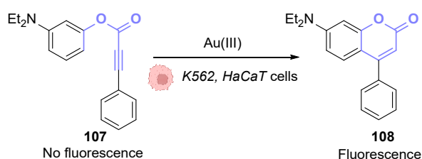
Fig. 37 Gold(III)-catalysed hydroarylation of non-fluorescent 107 into fluorescent coumarin. 88
