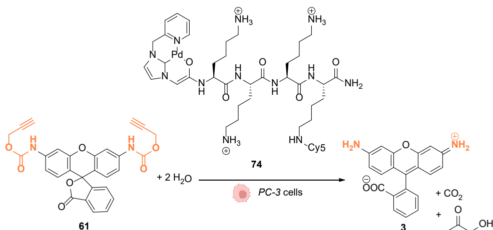
Fig. 28 Propargyl deprotection of a profluorescent probe by a discrete palladium complex inside PC-3 cancer cells. The ligand is linked to a polycationic cell penetrating peptide to favor cellular uptake. 70
