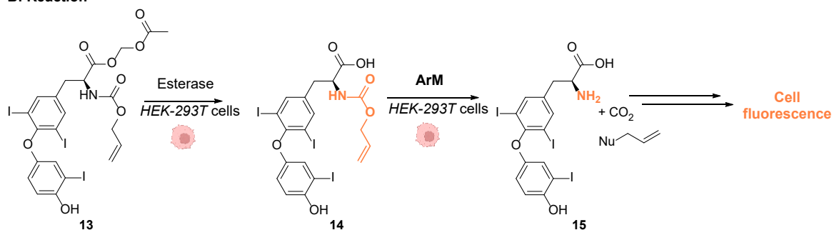
Fig. 5 (A) Assembly of a cell-penetrating Ru-based artificial metalloenzyme (ArM). The ruthenium catalyst and the fluorescent probe / cell penetrating peptide are both attached to biotin units interacting with streptavidin to create the artificial metalloprotein; (B) The ArM catalyses the Alloc deprotection of compound 14 , generating the hormone 15 . The HEK-293T cells have been modified to become fluorescent once 15 is liberated. 40
