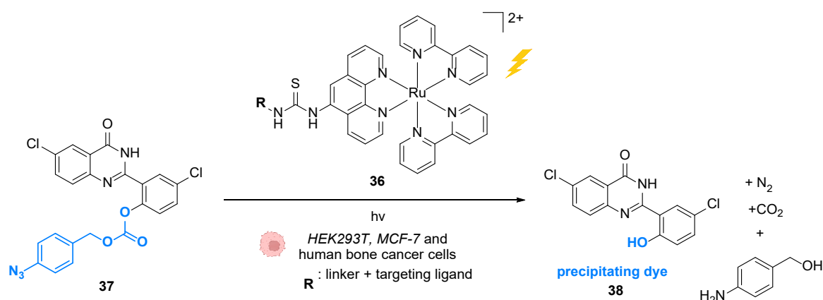
Fig. 14 Azide reduction of pro fluorescent probe inside different cells lines by the ruthenium(II) complex 36 , which is conjugated with a protein ligand R, allowing specific localisation of the reaction in targeted parts of the cell by two-photon excitation at 730 nm. 50
