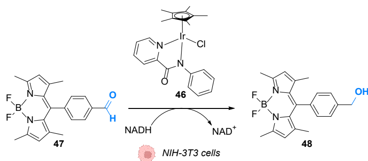
Fig. 19 Hydride transfer reaction catalysed by Ir III complex 46 inside NIH-3T3 mouse embryo fibroblast cells inducing intracellular fluorescence enhancement. 59
