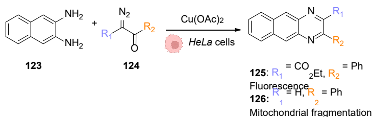
Fig. 43 Copper-catalysed metal carbene transfer reaction in HeLa cells for the assembly of quinoxalines such as the fluorescent compound 125 and the toxic compound 126 , capable of inducing mitochondrial fragmentation. 101
