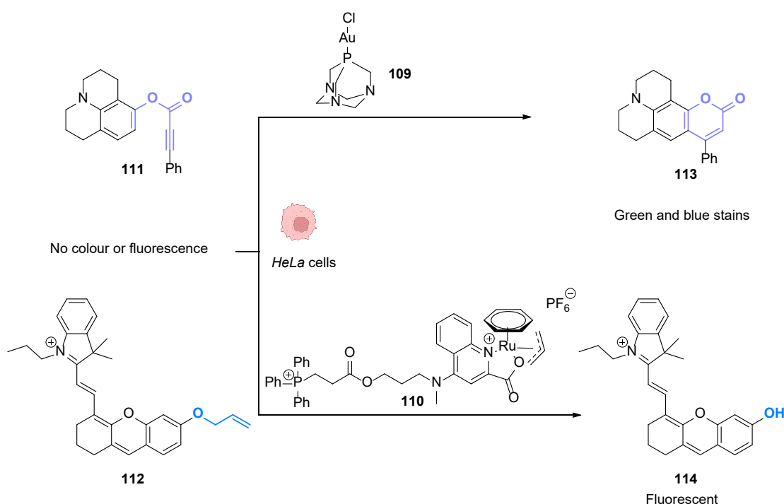
Fig. 38 Simultaneous Au I and Ru II catalysis inside HeLa cells. Gold-catalysed hydroarylation and allyl-deprotection catalysed by Ru. 89
