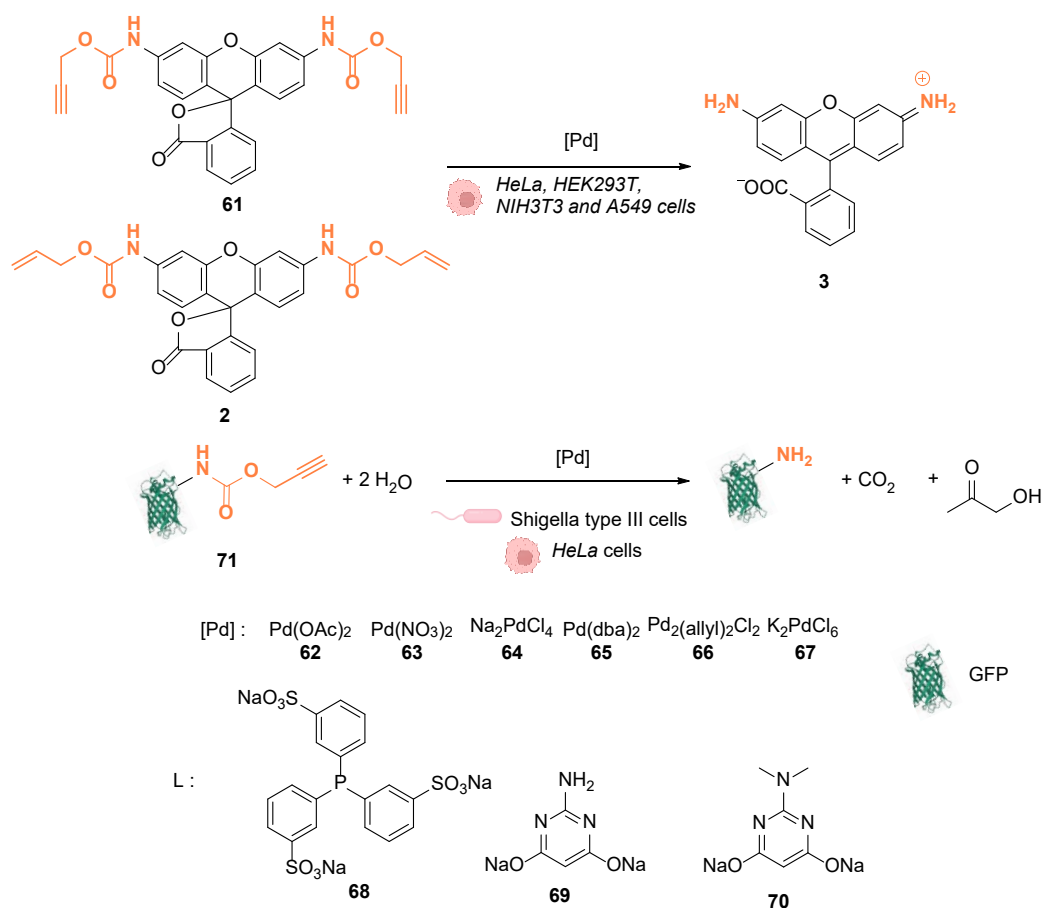
Fig. 26 Alloc and propargyloxycarbonyl deprotection of profluorophores by palladium complexes inside cells. 68
