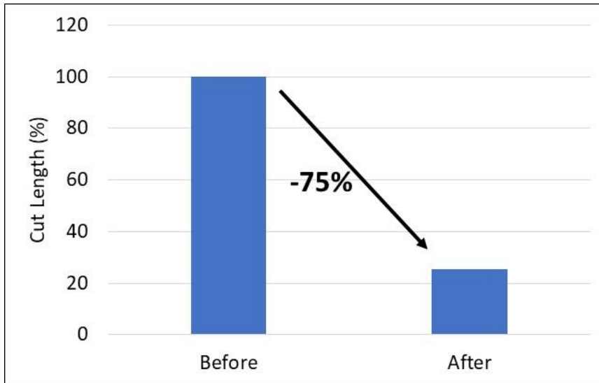
Fig. 26: Grade A Yield loss before and after maximizing the phase transformation on the run out table (e.g. minimizing phase transformation in the coil) and by homogenizing residual stress formation.
