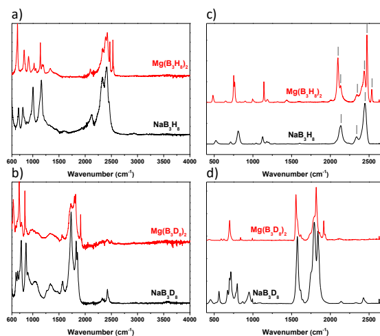
Figure 1. Comparison of FTIR spectra between \text{Mg}(\text{B}_3\text{H}_8)_2 and \text{NaB}_3\text{H}_8 (a) \text{Mg}(\text{B}_3\text{D}_8)_2 and \text{NaB}_3\text{D}_8 (b). Comparison of Raman spectra between \text{Mg}(\text{B}_3\text{H}_8)_2 and \text{NaB}_3\text{H}_8 (c) and \text{Mg}(\text{B}_3\text{D}_8)_2 and \text{NaB}_3\text{D}_8 (d).
