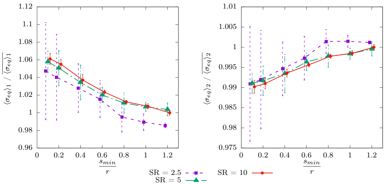
(b) contrast = 0.01, \overline{\langle \sigma_{eq} \rangle}_1 = 0.525 \text{ MPa}, \overline{\langle \sigma_{eq} \rangle}_2 = 29.1 \text{ MPa}
