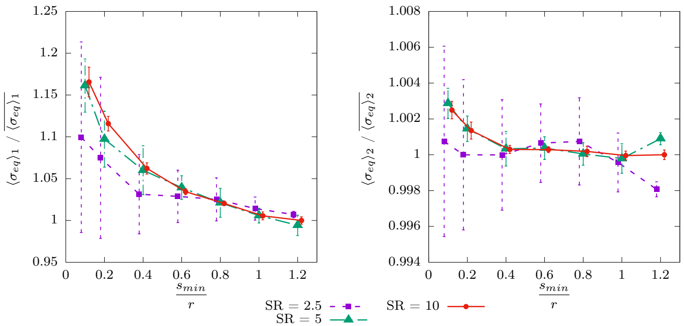
(a) contrast = 100, \langle \sigma_{eq} \rangle_1 = 75.1 \text{ MPa}, \langle \sigma_{eq} \rangle_2 = 37.0 \text{ MPa}
