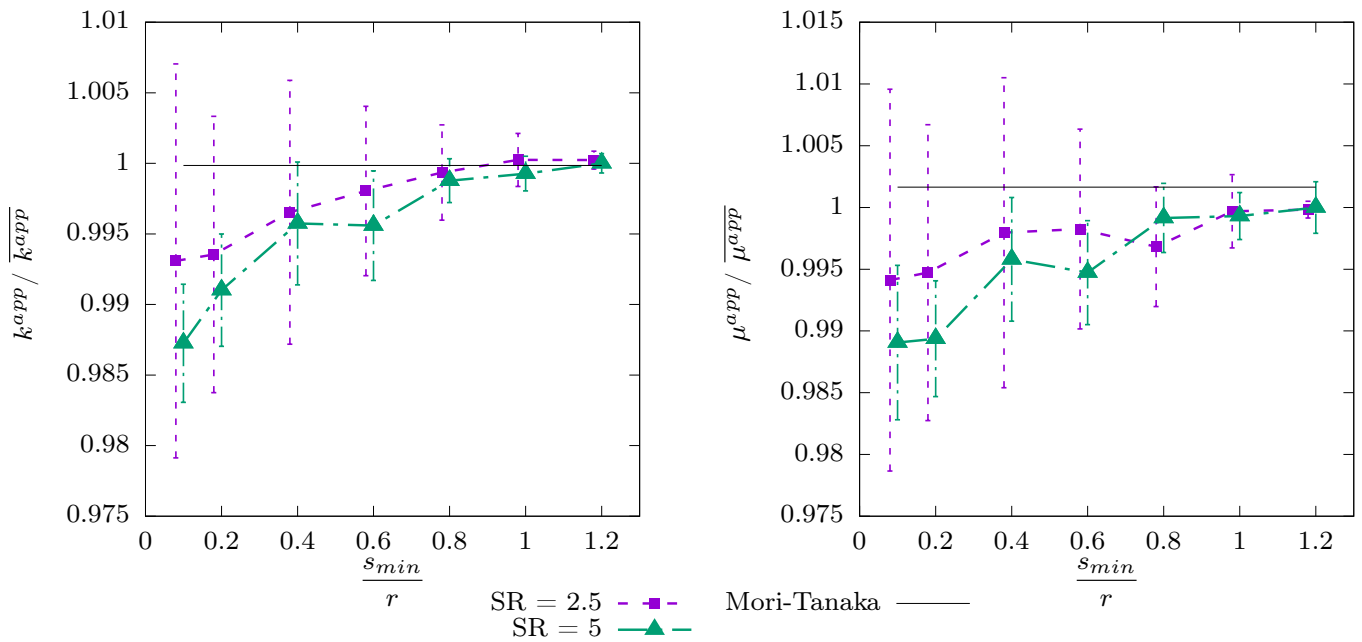
(b) contrast = 0.01, \bar{k}^{app} = 12.0 MPa, \bar{\mu}^{app} = 5.96 MPa
