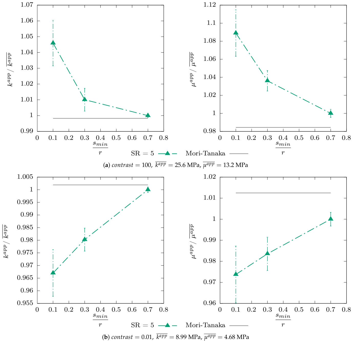
Figure 4. Mean values and standard deviations on the mean value for the apparent moduli as a function of the packing parameter s_{min}/r ( r = 10 \mu m ) for a volume fraction of inclusions f_v = 25.1\% .
