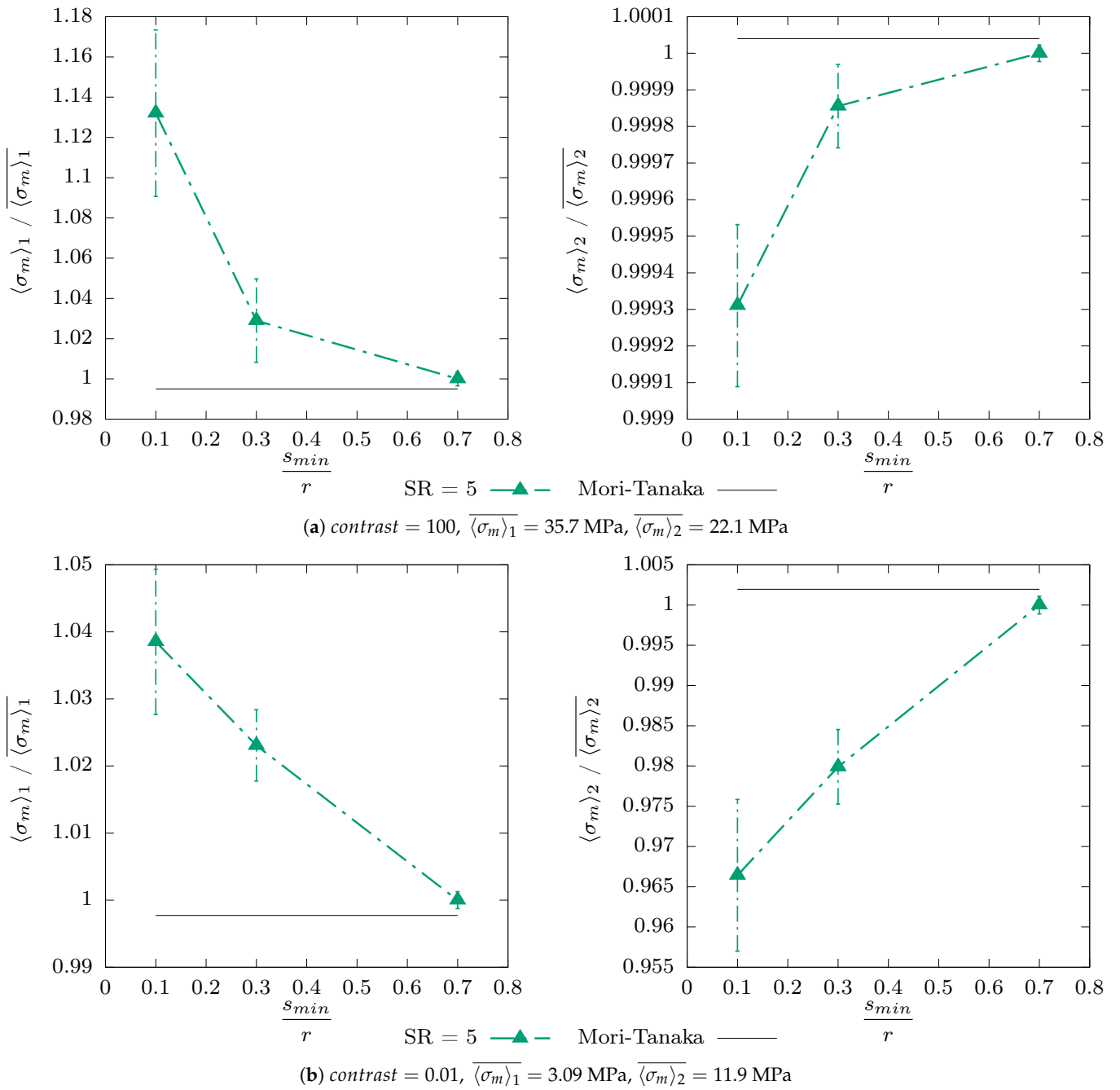
Figure A4. Mean values and standard deviations on the mean value for the first moment of hydrostatic stress by phase as a function of the packing parameter s_{min}/r ( r = 10 \mu\text{m} ) for a volume fraction of inclusions f_v = 25.1 \% .
