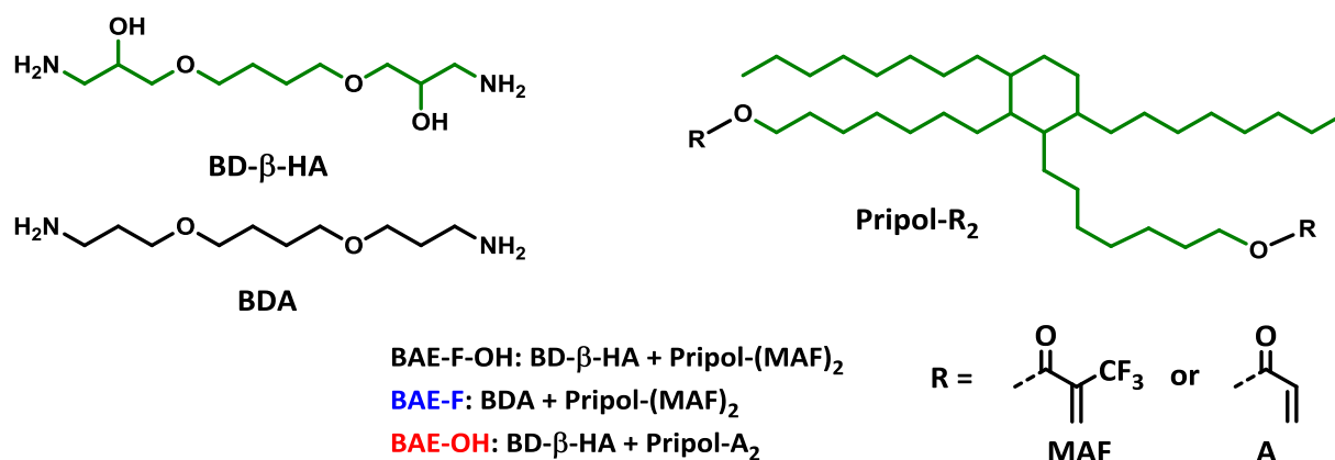
Figure 2. Monomer structures used for the synthesis of BAE networks, the green carbons correspond to biobased carbon.
