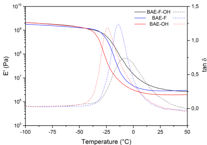
Figure 3. Storage modulus (full curves) and \tan(\delta) (dotted curves) for BAE-F-OH (black curve), BAE-F (blue curve) and BAE-OH (red curve).
