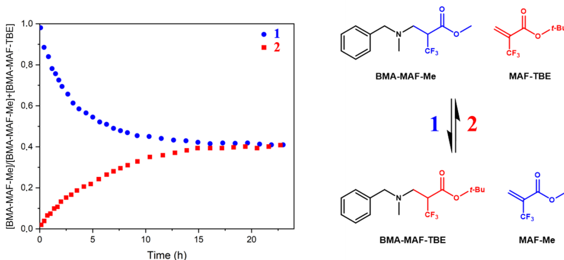
Figure 1. Kinetic monitoring of BMA-MAF-TBE and BMA-MAF-Me exchange reactions at 1M by ^{19}\text{F} -NMR in \text{DMF-d}_7 at 60 °C.
