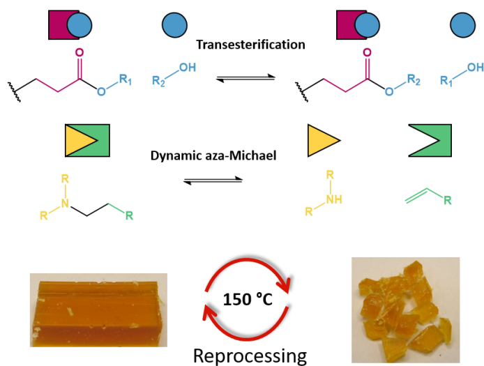
Figure 6. Schematic representations of BAE-F-OH, BAE-F and BAE-OH associated with their respective exchange reactions and reprocessing conditions.
