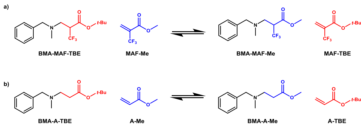
Scheme 2. Aza-Michael exchange reactions.
