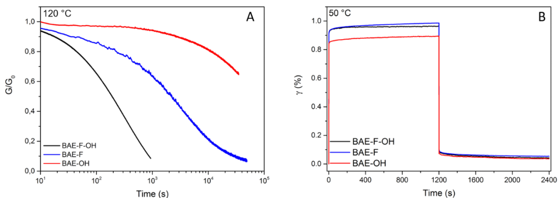
Figure 5. A) Normalized stress relaxation of BAEs at 120 °C for a 1 % strain B) Creep and recovery data for BAEs at 50 °C for an applied stress of 2 kPa.
