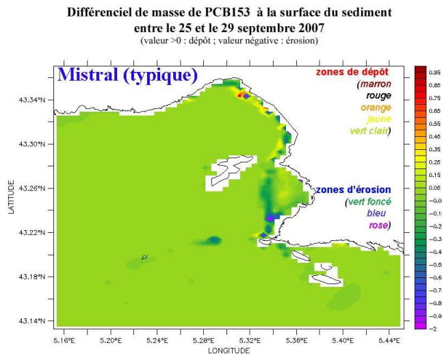
Figure 39: Zones of deposition/erosion during the typical Mistral in Sept 2007.
