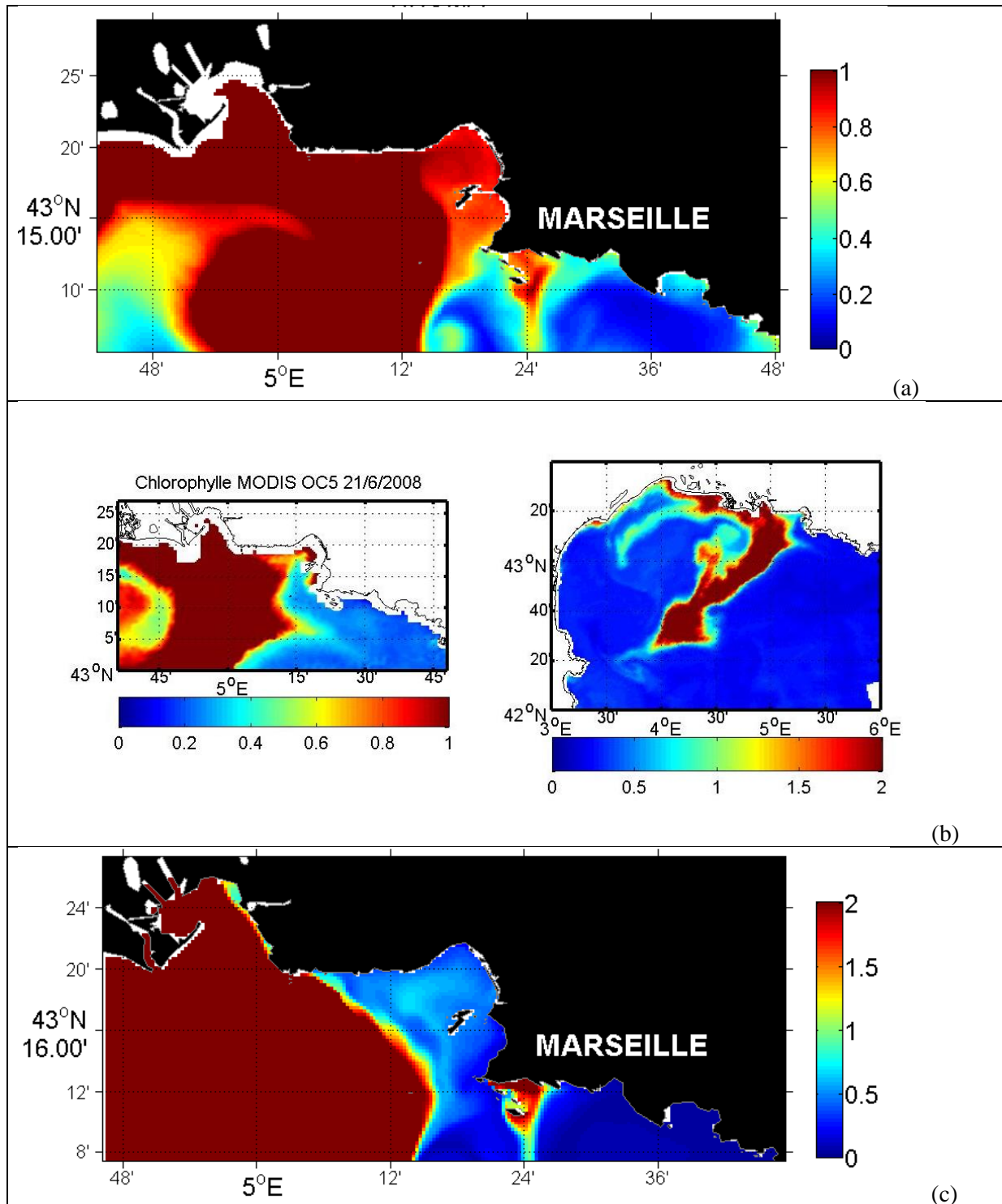
Figure 144: Maps for 21 June 2008 of (a) modelled surface chlorophyll concentrations (µg/L) (integrated over top 10m), (b) observed chlorophyll (µg/L) by MODIS (left: zoon on RHOMA area), and (c) modelled surface nitrate (µmol/L).
