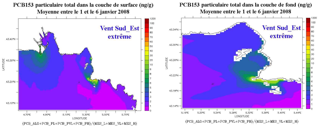
Figure 81: Mean particulate CB153 (ng/g) at the surface and sea bed between 1 and 6 Jan 2008
