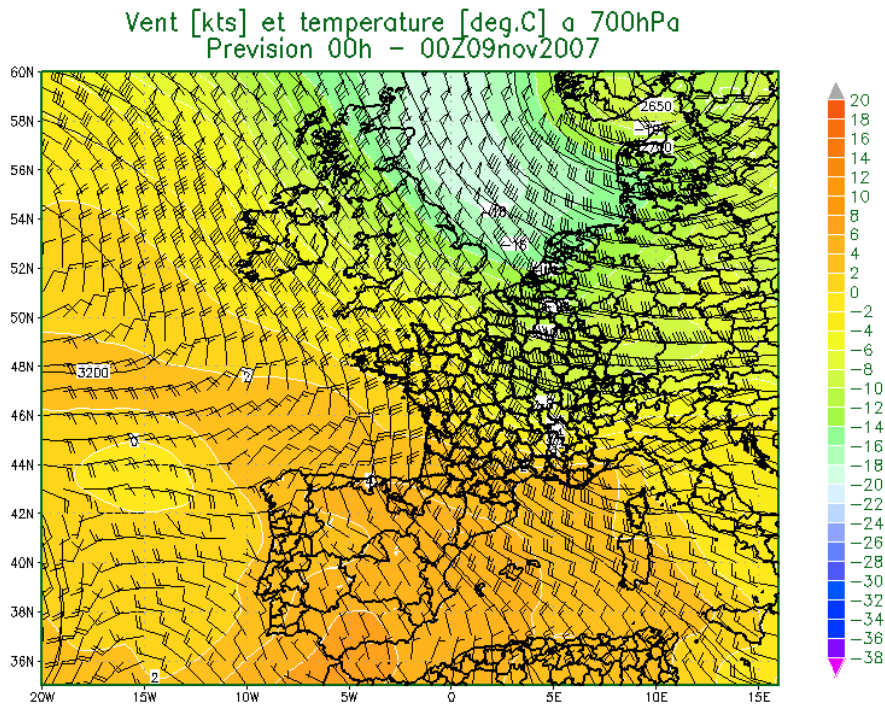
Figure 41: Wind (kts) and temperatures (°C - colour bar) at 700hPa on 9 Nov 2007 at 00h.
