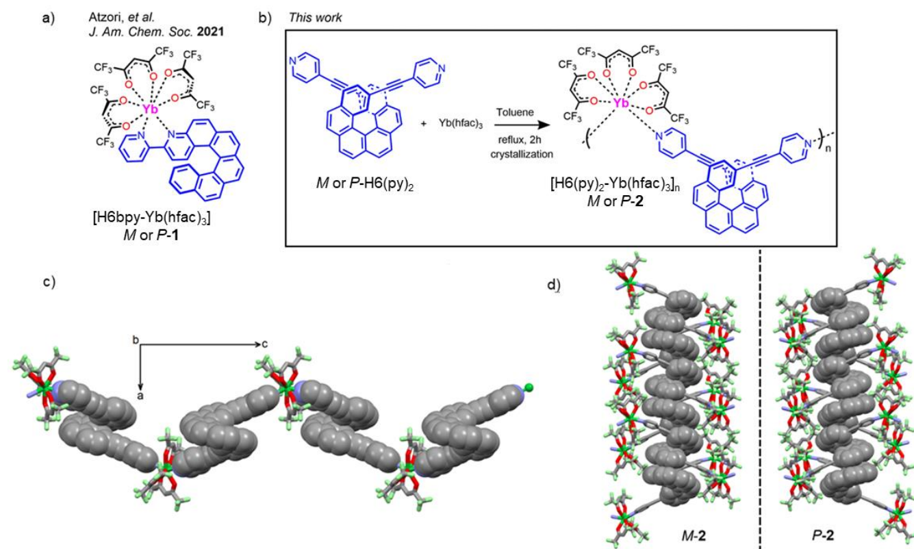
Figure 1. a) Molecular structure of [H6bpy-Yb(hfac) 3 ] 1 , b) chemical reaction for the formation of [H6(Py) 2 Yb(hfac) 3 ] n 2 , c) X-ray structure of M - 2 along the c axis with H6(Py) 2 ligand and Yb(hfac) 3 moieties respectively drawn in capped sticks and spacefill representations, and d) supramolecular arrangement of the two enantiomers along the a axis.
