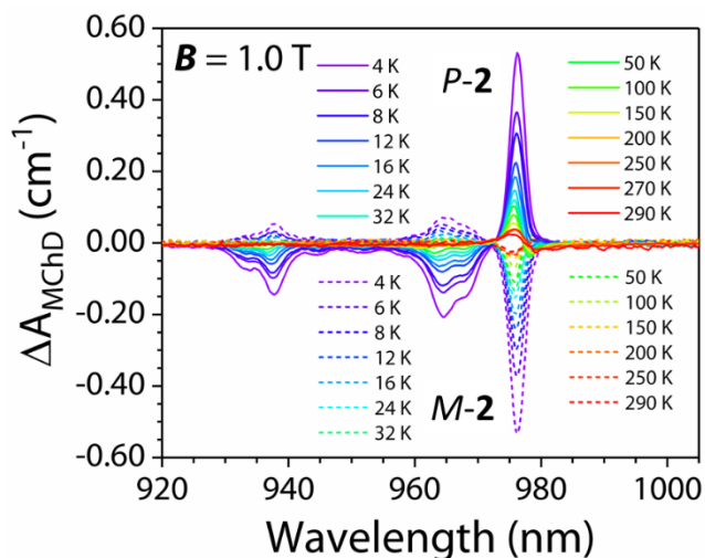
Figure 6. Temperature variation (see legend) of MChD spectra (920–1005 nm) of P-2 and M-2 recorded on an oriented single crystal under an applied magnetic field B = \pm 1.0 T.
