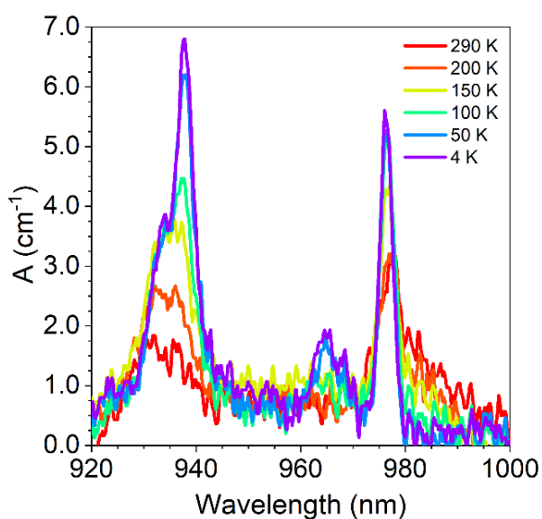
Figure 3. Temperature variation (selected temperature, see legend) of the absorption spectrum (920-1000 nm) for a single crystal of (P)-2 measured with the unpolarized light wavevector propagating along the c crystallographic axis.
