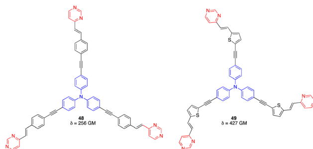
Fig. 23 Structures of octupolar arylvinylnitrides 48 and 49.
