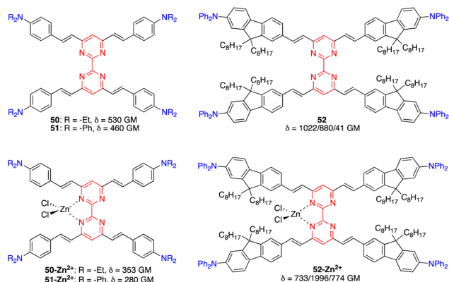
Fig. 24 Structures of bipyrimidine chromophores 50–52.
