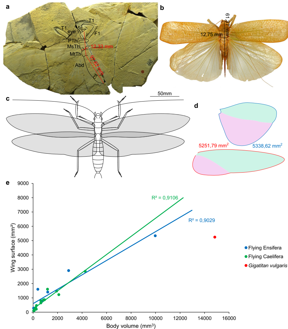
Fig. 6 Flying ability of Gigatitan vulgaris . a Specimen PIN 2240/4593; PTh prothorax, MsTh mesothorax, MtTh metathorax, Abd abdomen, Md mandible, F1 profemora, T1 protibia. b Pseudophyllanax imperialis , one of largest extant flying Orthoptera. c Reconstruction of Gigatitan vulgaris . d Hind wings of Pseudophyllanax imperialis (top, from (b) ) and Gigatitan vulgaris (bottom, after 6 ) with areas; note the differences in size of the vannus (in pink). e Wing surface plotted against body volume for several extant flying Orthoptera and Gigatitan vulgaris . Gigatitan seems too heavy to be able to fly actively. a-d : same scales.
