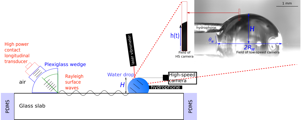
FIG. 1. Sketch of the experimental setup. A 10.0 \mu\text{l} water drop deposited on a glass slab is irradiated with a harmonic progressive Rayleigh wave generated using a contact longitudinal transducer mounted on a wedge. The slab edges are surrounded by PDMS, which ensures efficient attenuation of SAW echoes in the glass slab. A needle hydrophone, whose tip is brought into contact with the liquid surface, measures the intracavity pressure. Full pictures of the slowly evaporating drop are taken at 30 fps using a camera (main picture at top right of the figure), while the oscillations of the drop-free surface in a narrow field close to its apex (red frame on the picture) are recorded at 1000 fps using a high-speed camera (narrow picture on the left of the main picture). A laser vibrometer pointing close to the apex is used for measuring low-amplitude surface oscillations in independent experiments dedicated to the characterization of the unstable surface eigenmode, which are presented in [33].
