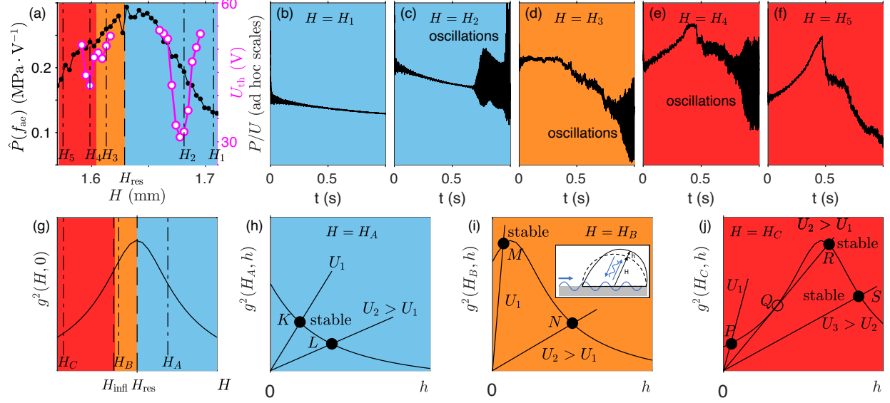
FIG. 5. (a) Left scale, joined black symbols: H -dependent pressure response \hat{P} at excitation frequency f_{ae} . Right scale, joined open magenta symbols: instability threshold voltage U_{th} vs H . The blue area corresponds to H > H_{res} (blue detuning). The orange and red areas correspond to H < H_{res} (red detuning). (b-f) Time evolution of the cavity pressure response P/U = \hat{P} during a U -ramp for four different values of the drop height H = H_i , i = 1 to 4, as defined in (a). Oscillation episodes are visible in (c-e). (g) Schematic variation of the square of the pressure response \hat{P}^2 = P^2/U^2 = g^2 vs H . (h-j) Schematic variation of g^2 vs resonator lengthening h (see inset of (i)) for three different values of the drop height H = H_X , X = A, B, C , as defined in (g). Inset of (i): sketch of the drop quasistatic deformation.
