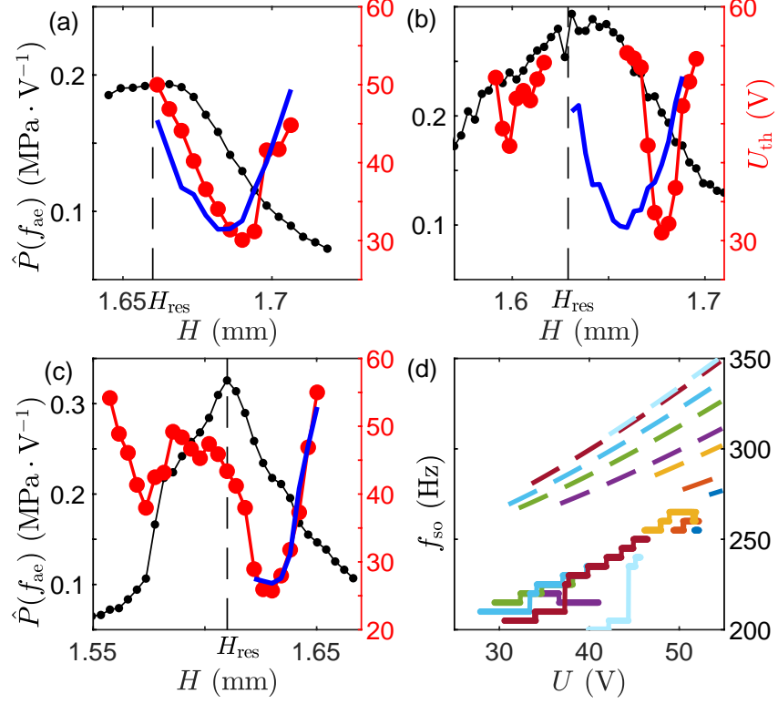
FIG. 4. (a-c) Left scale, joined black symbols: H -dependent pressure response \hat{P} at excitation frequency f_{ae} . Right scale, joined red symbols: instability threshold voltage U_{th} vs H . Blue curve: best fit of U_{th}(h) by Eqs. (4, 6). (d) Solid curves: measured surface oscillation frequency f_{so} vs U ( \geq U_{th} ) for several values of H . Dashed curves: corresponding predictions from Eq. (7).
