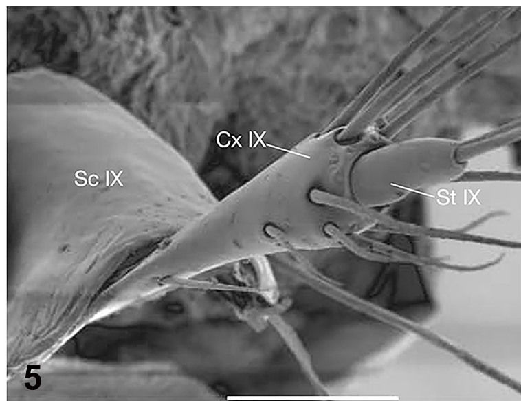
Figures 4–5. Ochodaeidae, female terminalia. 4) Nothochodaeus minotaurus Huchet, new species (holotype), right part. 5) Ochodaeus miliaris Klug, 1832, with stylus IX present (after Dupuis, 2005) (Cx: coxite; Ep: epipleurite; Sc: subcoxite; Te: tergite). (Fig. 5: photo courtesy of F. Dupuis; scale = 100 \mu m).
