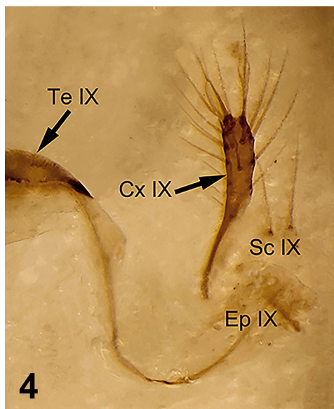
Figures 4–5. Ochodaeidae, female terminalia. 4) Nothochodaeus minotaurus Huchet, new species (holotype), right part. 5) Ochodaeus miliaris Klug, 1832, with stylus IX present (after Dupuis, 2005) (Cx: coxite; Ep: epipleurite; Sc: subcoxite; Te: tergite). (Fig. 5: photo courtesy of F. Dupuis; scale = 100 \mu m).
