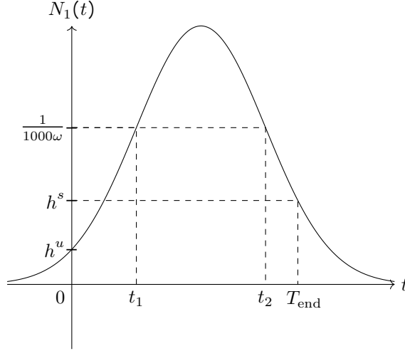
Figure 17: Graph of t \mapsto N_1(t) . T_{\text{end}} = \tau_{\omega, h^s}(\mathcal{P}_{\omega, h^u}^u) .
