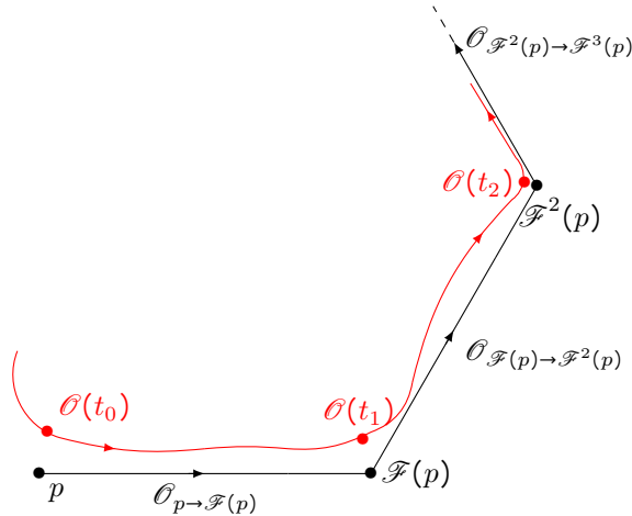
Figure 2: Schematic representation of the first part of a heteroclinic chain shadowed by a type IX orbit in \mathcal{B}^+ .
