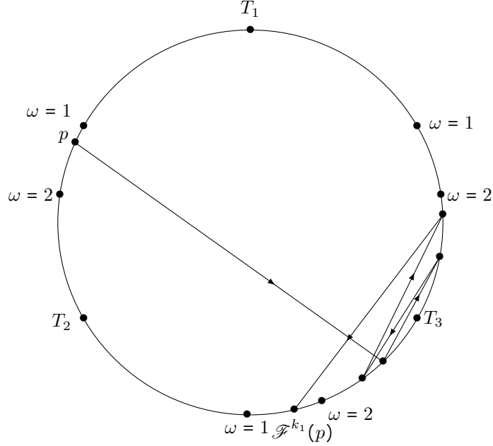
Figure 5: First era of the heteroclinic chain starting at p , represented in projection on the plane containing the Kasner circle.
