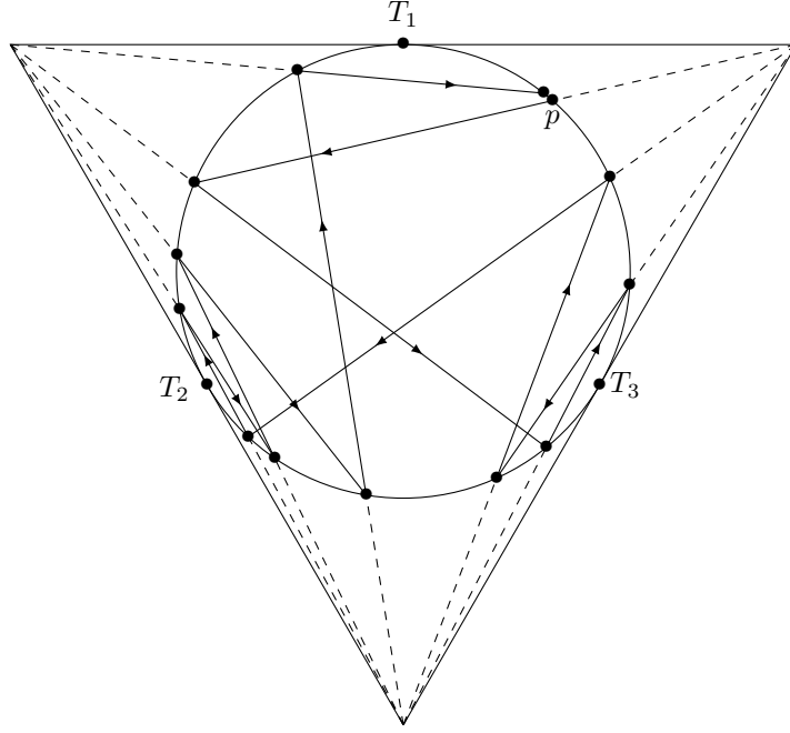
Figure 10: The Kasner map is chaotic.
