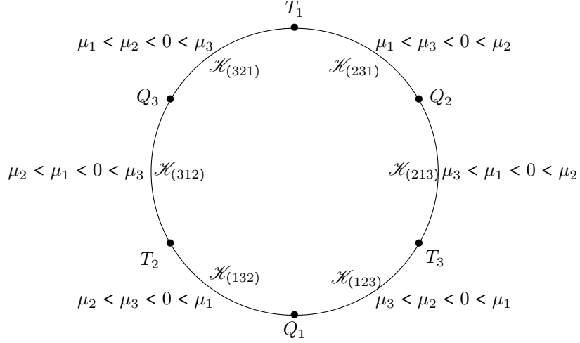
Figure 6: Order of the eigenvalues.
