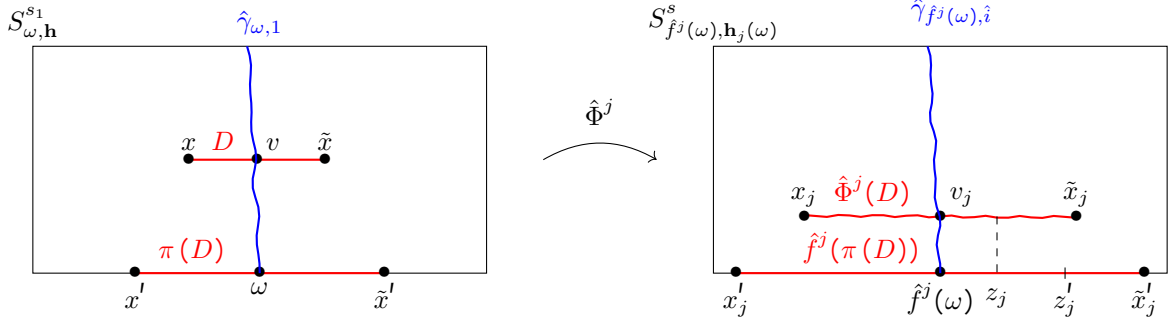
Figure 25: Iteration of the two horizontal segments. To avoid clutter, we denote \hat{i} = \hat{i}(\hat{f}^{j-1}(\omega)) .
