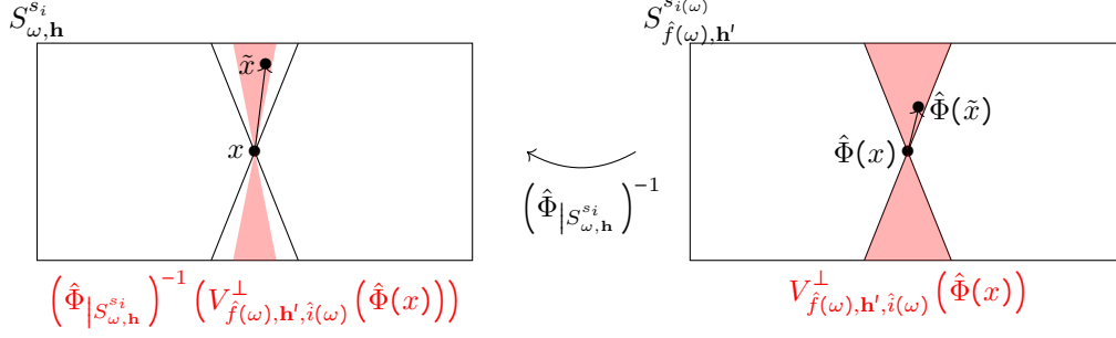
Figure 19: Backward invariance of the transverse cone field.
