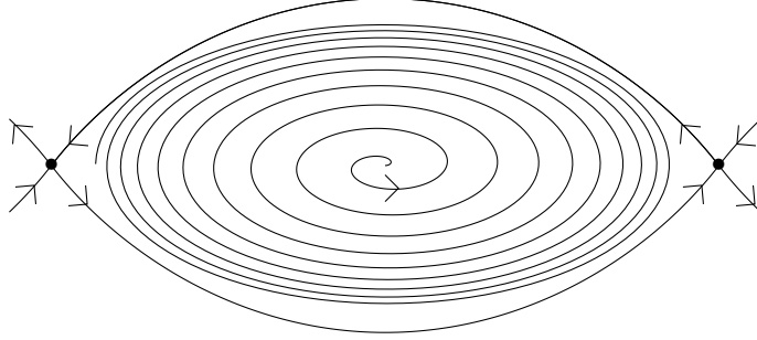
Figure 3: Bowen's eye attractor.
