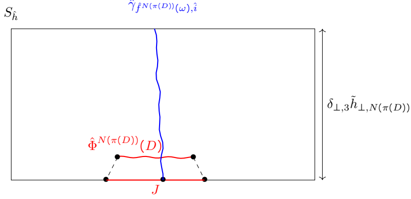
Figure 26: \pi(\hat{\Phi}^{N(\pi(D))}(D)) \subset J with |J| \leq |\hat{\Phi}^{N(\pi(D))}(D)| + \delta_{\perp, 3\tilde{h}_{\perp, N(\pi(D))}} . To avoid clutter, we denote \hat{i} = \hat{i}(\hat{f}^{N(\pi(D))^{-1}}(\omega)) .
