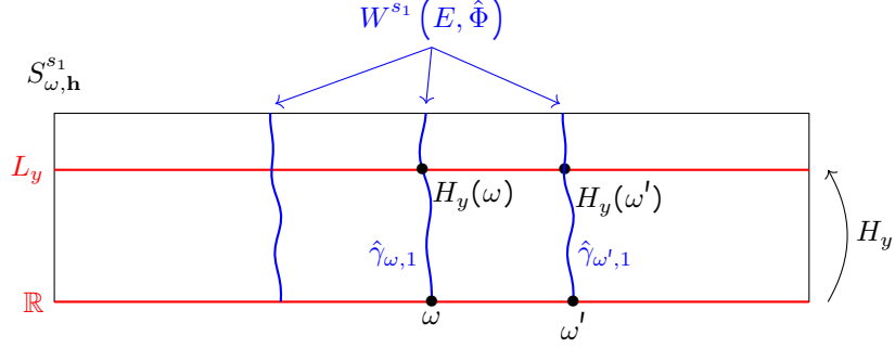
Figure 22: The map H_y .
