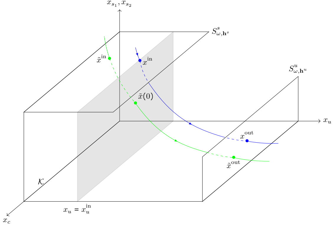
Figure 16: A pair of (S_{\omega, \mathbf{h}^s}^s, S_{\omega, \mathbf{h}^u}^u) -synchronized orbits.
