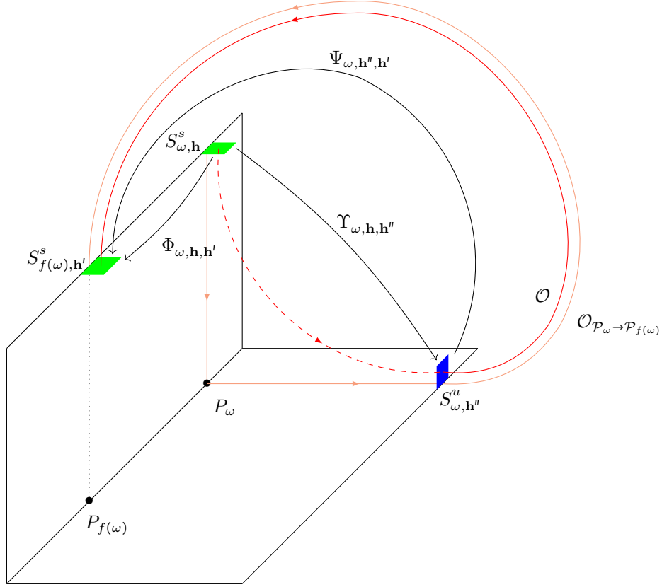
Figure 14: A type IX orbit \mathcal{O} (in red) traveling between the section S_{\omega, \mathbf{h}}^s and the section S_{f(\omega), \mathbf{h}'}^s . During this travel, the orbit \mathcal{O} stays close to a piece of heteroclinic chain (in melon) passing through the point \mathcal{P}_{\omega} . If the parameters \mathbf{h} , \mathbf{h}' and \mathbf{h}'' are well-chosen (roughly speaking, \mathbf{h}' must be small enough, \mathbf{h}'' much smaller than \mathbf{h}' and \mathbf{h} much smaller than \mathbf{h}' ; explicit bounds will be given in the next sections), the orbit \mathcal{O} will first cross the section S_{\omega, \mathbf{h}''}^u and then cross the section S_{f(\omega), \mathbf{h}'}^s .
