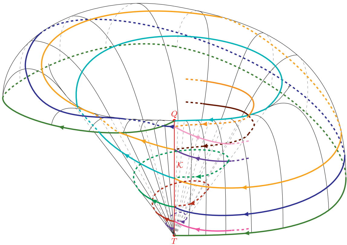
Figure 11: Half of the quotient Mixmaster attractor and some type II orbits.
