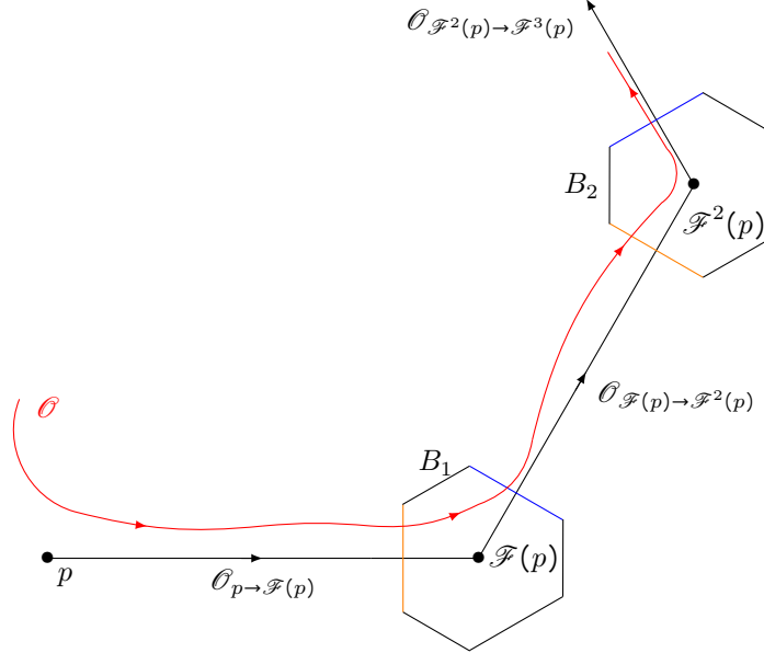
Figure 4: The orbit \mathcal{O} successively enters the neighbourhoods B_1, B_2, \dots . Each time it passes inside one of these neighbourhoods, it gets much closer to the heteroclinic chain starting at p , due to the super-linear contraction.
