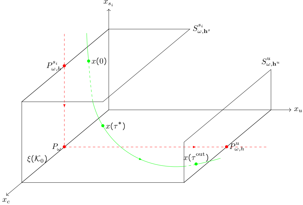
Figure 15: Notations for local shadowing.
