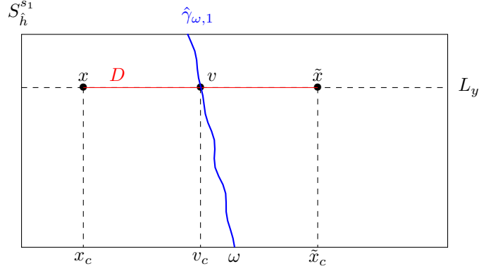
Figure 24: Segment D centered above \omega with its end points.
