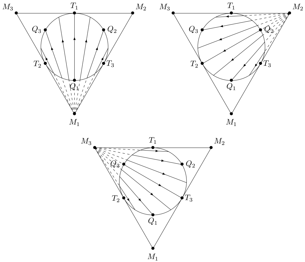
Figure 8: Projections on the (\Sigma_1, \Sigma_2, \Sigma_3) -plane of type II orbits contained in \mathcal{B}_{\text{II}}^1 , \mathcal{B}_{\text{II}}^2 and \mathcal{B}_{\text{II}}^3 (left to right, top to bottom).
