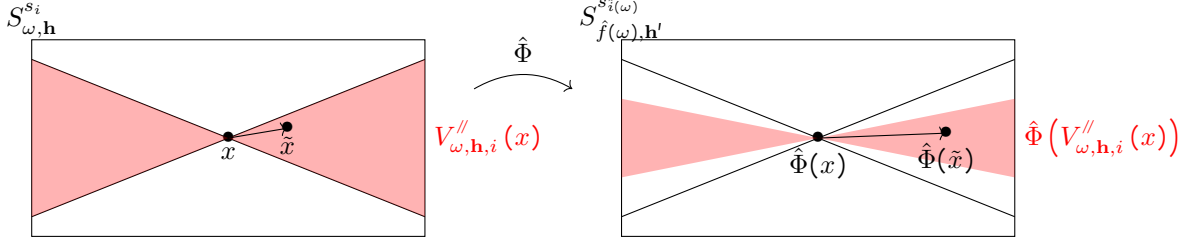
Figure 18: Forward invariance of the tangential cone field.
