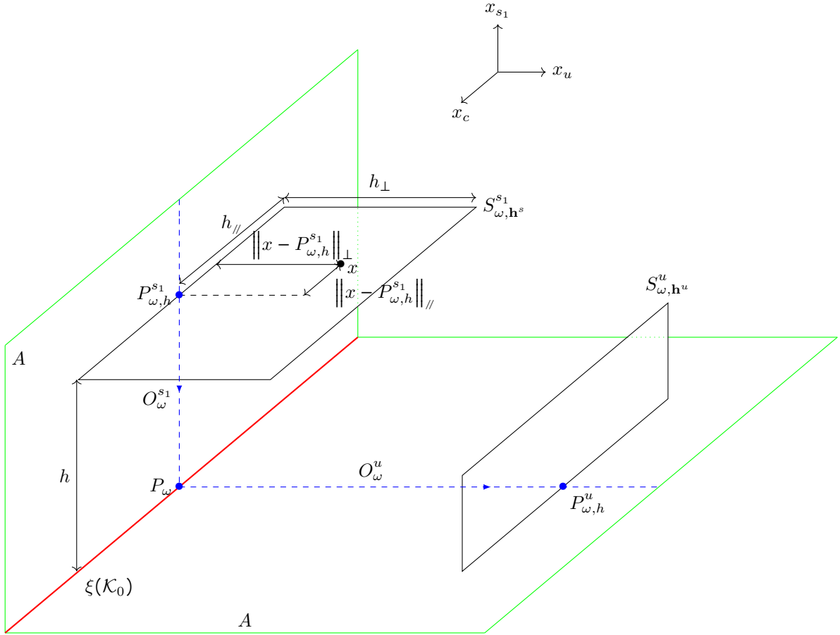
Figure 12: Sections S_{\omega, h}^{s_1} and S_{\omega, h}^u . We omit the x_{s_2} -direction since we cannot draw in four dimensions. The Mixmaster attractor A is represented in green. The Kasner interval \xi(\mathcal{K}_0) is represented in red. The type II orbits arriving and starting at P_{\omega} are represented in blue.
