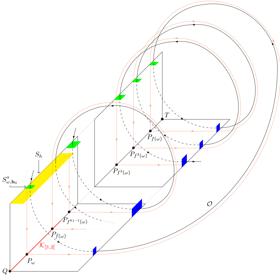
Figure 13: A type IX orbit \mathcal{O} (in black) traveling close to the first era of the heteroclinic chain starting at P_\omega (in melon), where \omega = [1; k_1, k_2, \dots] . The local sections S_{\omega, \mathbf{h}_0}^s, S_{f(\omega), \mathbf{h}_1}^s, \dots, S_{\bar{f}(\omega), \mathbf{h}_{k_1}}^s are represented in green, while the local sections S_{\omega, \mathbf{h}_0}^u, S_{f(\omega), \mathbf{h}_1}^u, \dots, S_{\bar{f}(\omega), \mathbf{h}_{k_1}}^u are represented in blue. The era transition map \bar{\Phi}_{\omega, \mathbf{h}_0} encodes the travel of the orbit \mathcal{O} between the local section S_{\omega, \mathbf{h}_0}^s and the global section S_h (in yellow). One can decompose the era transition map into several epoch transition maps, encoding the travel of the orbit \mathcal{O} between two consecutive green sections.
