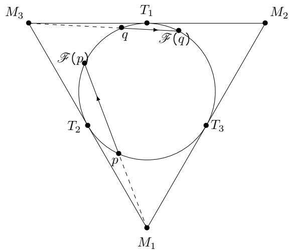
Figure 9: The Kasner map.
