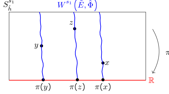
Figure 23: The projection map \pi .
