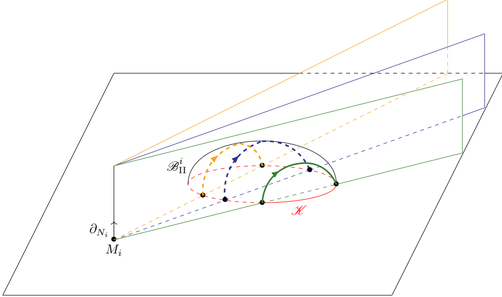
Figure 7: Type II orbits contained in \mathcal{B}_{\text{II}}^i .
