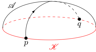
Figure 1: A type II orbit connecting two points of the Kasner circle \mathcal{H} .
